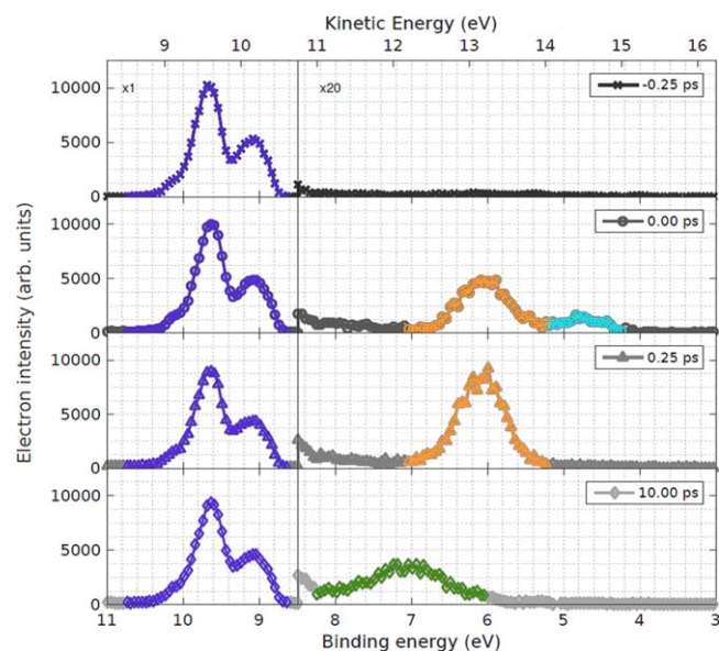
Figure 10. Valence photoelectron spectra of acetylacetonone as a function of pump–probe delay. Reprinted by permission from Springer Nature Customer Service Centre GmbH: Nature Communications [95] 2018 CC-BY 4.0.
