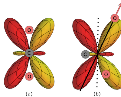
FIG. 3: (color online). a) One component of the doubly degenerate {}^2\Pi_u electron attachment entrance amplitude for the 4 eV shape resonance in CO_2 for equilibrium geometry. b) The same entrance amplitude as Fig. 3a, rotated with respect to the molecular axis to simulate non-axial recoil, as discussed in the text.
