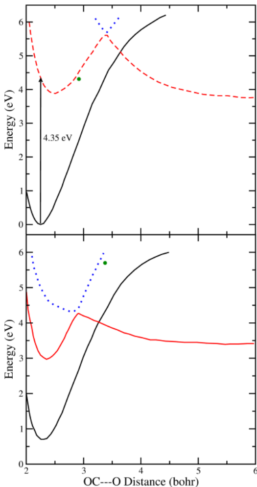
FIG. 6: (color online). Potential curves of neutral \text{CO}_2 and the shape- and Feshbach anion states, showing the avoided crossing between the two resonance states. No adjustment of the neutral and anion curves was made. Upper: Linear geometry; the point near 3 bohr shows the position of the crossing when the OCO angle is 140 degrees. Lower: O-C-O angle is 140 degrees; the point near 3.4 bohr shows the position of the crossing when the OCO angle is 180 degrees.
