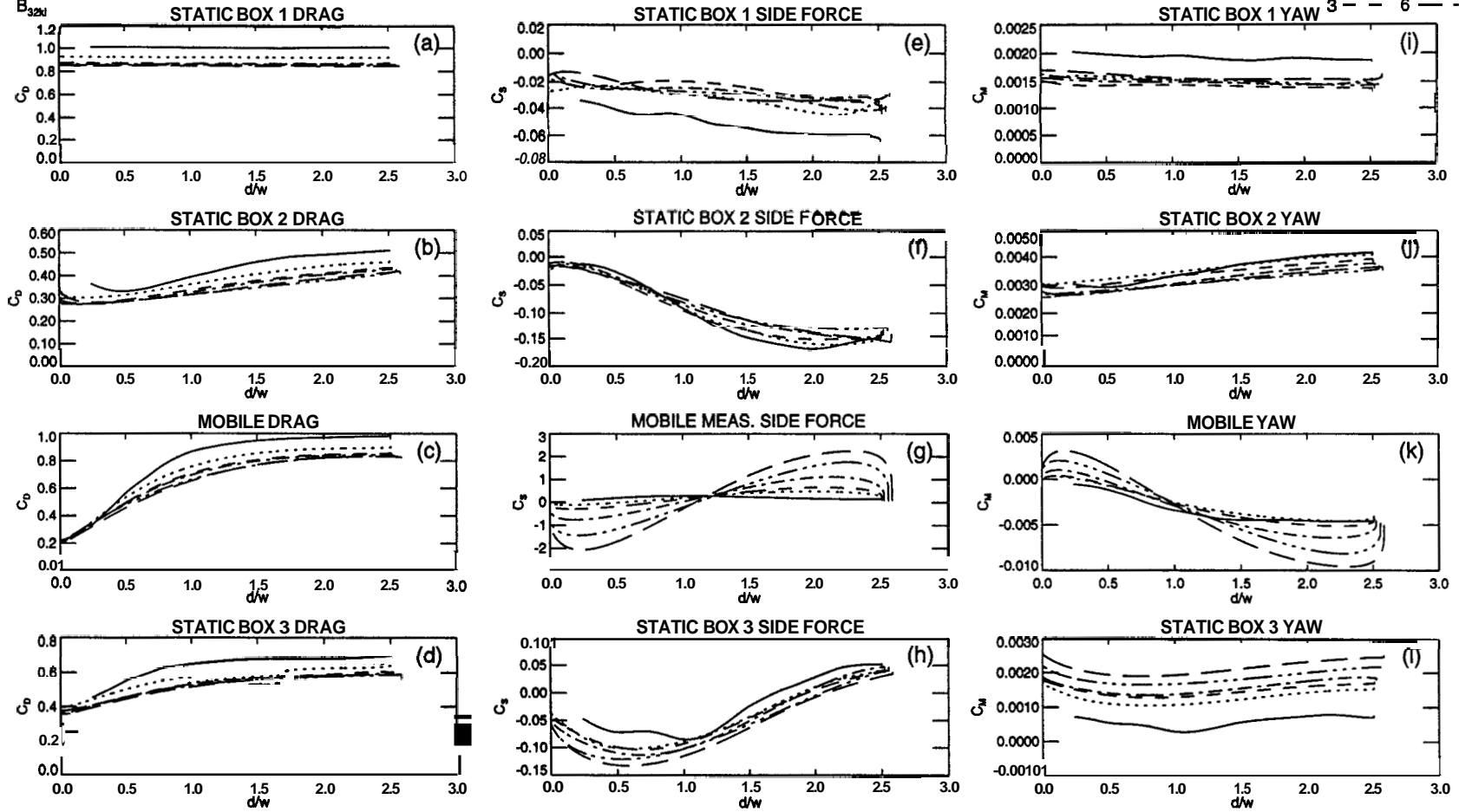
Figure 6.19: Effect of acceleration, boxes (position = 3, separation = 0.4l , motion inward). The drag [frames (a)-(d)], side force [frames(e)-(h)], and yawing moment [frames(i)-(l)] coefficients on each box are shown with respect to lateral displacement of the mobile box. The different lines represent the six acceleration profiles of the mobile box.
