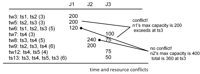
Figure 8: Time and Resource Conflicts
