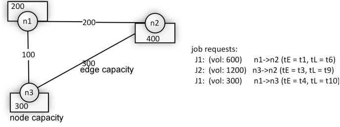
Figure 1: Sample Problem Definition
