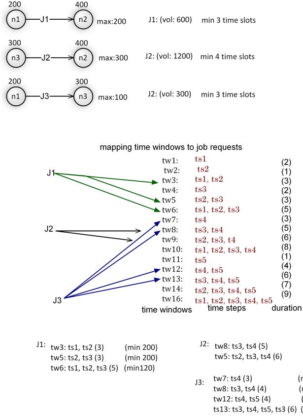
Figure 5: Mapping Jobs to Time Windows
