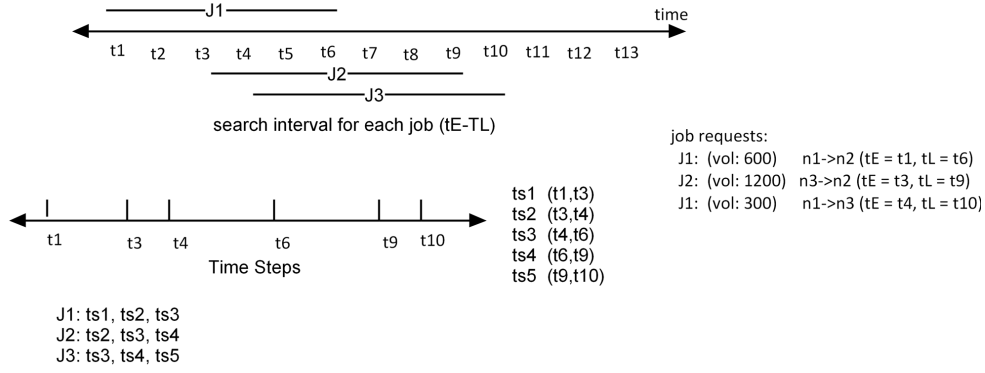
Figure 4: Time Steps and Search Interval
