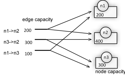
Figure 2: Node and Link - Resource Constraints
