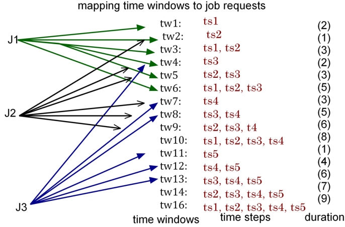
Figure 3: Time Windows
