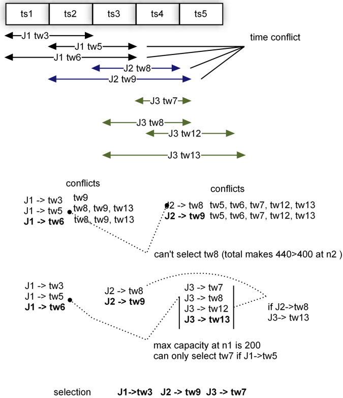
Figure 10: Assigning Jobs to Time Windows
