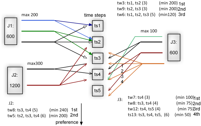
Figure 7: Time Conflicts
