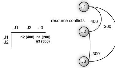
Figure 9: Resource Conflicts
