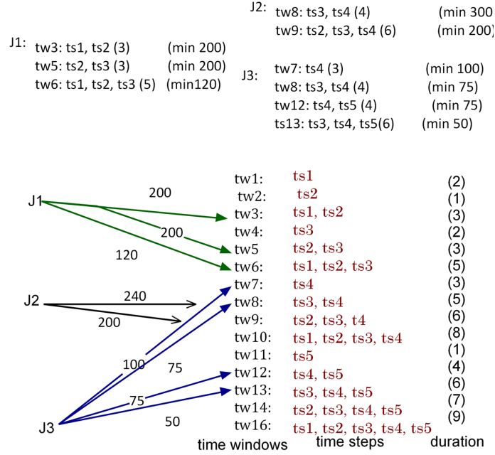
Figure 6: Minimum Capacity required for each Time Window
