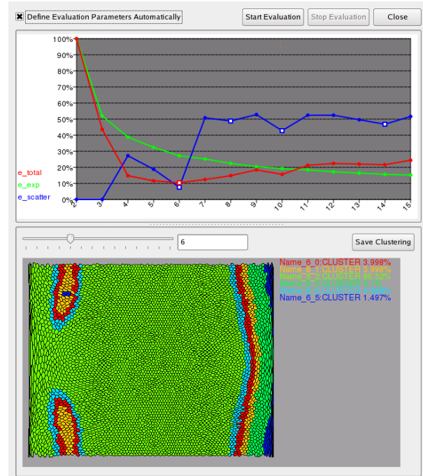
Figure 4.14: GUI for the evaluation of the number of clusters k . At the top, a plot of the cluster evaluation functions \epsilon_{\text{scatter}} , \epsilon_{\text{exp}} , and \epsilon_{\text{total}} is shown. After the evaluation is completed the suggested values are marked in the plot and a preview of the suggested clustering is shown at the bottom in an Unrolled View. Using a slider the user can and scroll through the evaluated clusterings by changing k and save any clustering of interest to cluster management.
