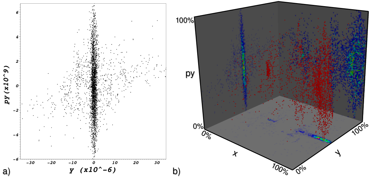
Figure 2.3: a) Illustration of a two-dimensional (2D) scatter plot in (y, p_y) space of all accelerated particles (i.e., particles with p_x > 10^{10} ) at a single time step of a laser wakefield particle accelerator (LWFA) simulation in 2D (see Section 3.2 for an introduction to LWFAs). b) Illustration of a three-dimensional (3D) scatter plot in (x, y, p_y) space of the same data as shown in a. The data points of the scatter plot (each representing a particle) are shown via red spheres. The corresponding 2D histograms are shown in color on the outside surfaces of the cube defined by the scatter plot (gray/blue=low, green=medium, and red=high particle density).
