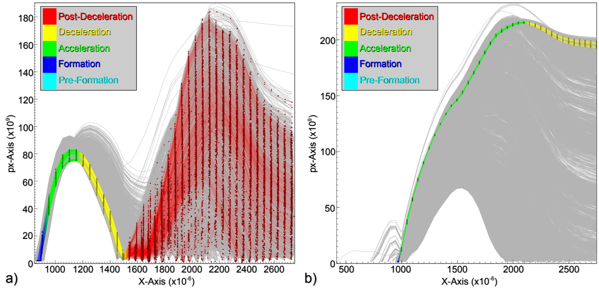
Figure 5.33: a) Temporal phases of the first bunch. b) Temporal phases of the second bunch. Both figures show the paths of all candidate particles of the according bunch in gray. The reference particles and their paths are shown in addition colored according to the different beam-phases. The second bunch (b) does not show a post-deceleration phase because the simulation terminated before the bunch had completed deceleration.
