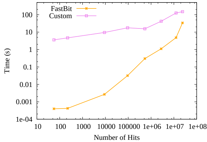
Figure 5.13: Timings for serial processing of particle identifier queries.
