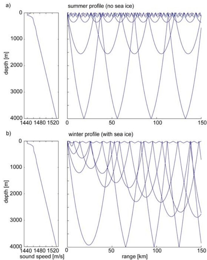
Figure 1.2. Sound propagation characteristics in the Southern Ocean during (a) summer and (b) winter conditions with associated sound speed profile characteristics.
