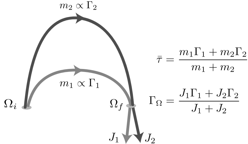
Figure 1. A simple two-pipe model to illustrate the distinction between reservoir mean residence time \bar{\tau} and mean age at exit \Gamma_\Omega : \bar{\tau} is a mass-weighted mean over the entire fluid domain, while \Gamma_\Omega is a mean for which the flow rates provide the weights. If the flow rates J_1 and J_2 in the two pipes (one-way fluxes in the general case) are equal, then mean age at exit on \Omega_f is \Gamma_\Omega = (\Gamma_1 + \Gamma_2)/2 , while the mass-weighted mean residence time of all fluid elements in the pipes is given by \bar{\tau} = (\Gamma_1^2 + \Gamma_2^2)/(\Gamma_1 + \Gamma_2) = \Gamma_\Omega + 2\Delta^2/\Gamma_\Omega , where \Delta measures the spread between \Gamma_1 and \Gamma_2 . For details, see text.
