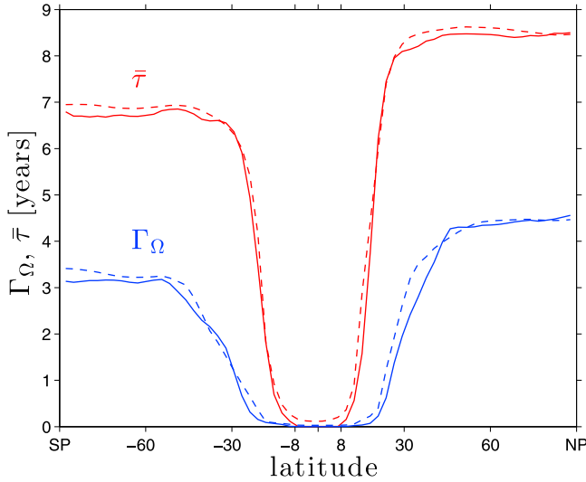
Figure 2. Red lines: the mean residence time \bar{\tau} of air that entered the stratosphere between 8^{\circ}\text{S} and 8^{\circ}\text{N} ( \Omega_{\text{EQ}} air) and that exits at the latitude of the abscissa. Blue lines: the corresponding mean age on exit, \Gamma_{\Omega} . Solid lines indicate the quantity was computed using the one-way flux-density distribution \mathcal{J} , while dashed lines indicate that the limit of moment ratios was used.
