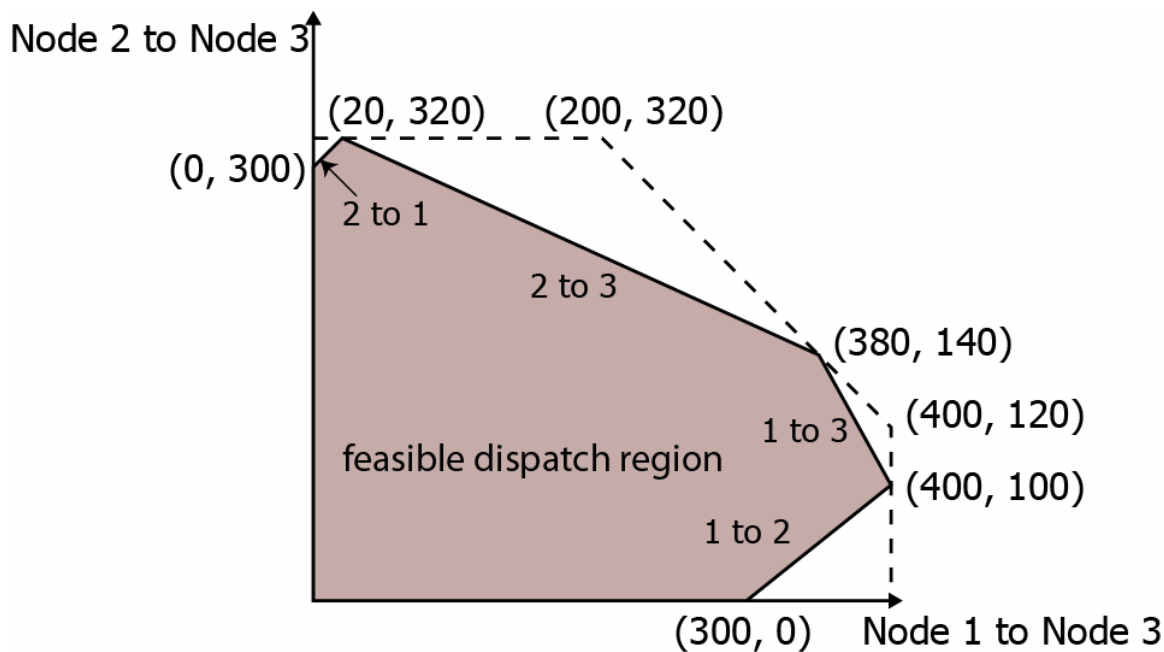
Figure 1-3 Nomogram of a Three-Node Example
