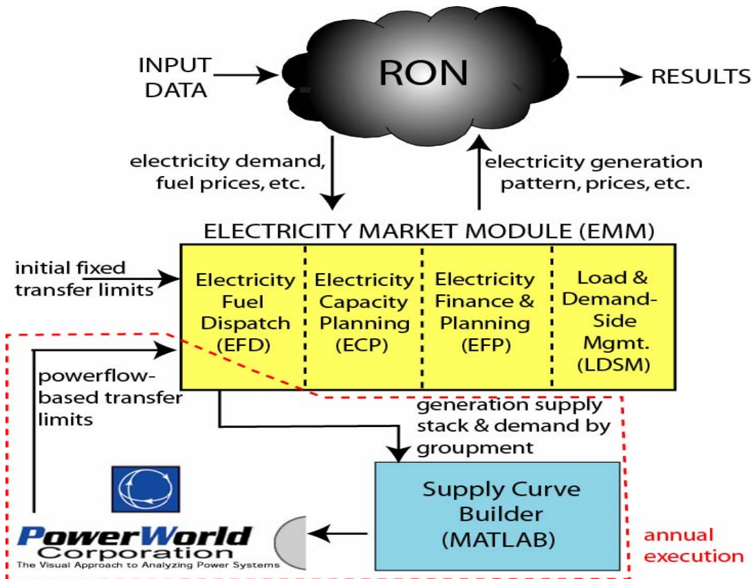
Figure 2-1 The RON Power Flow Model
