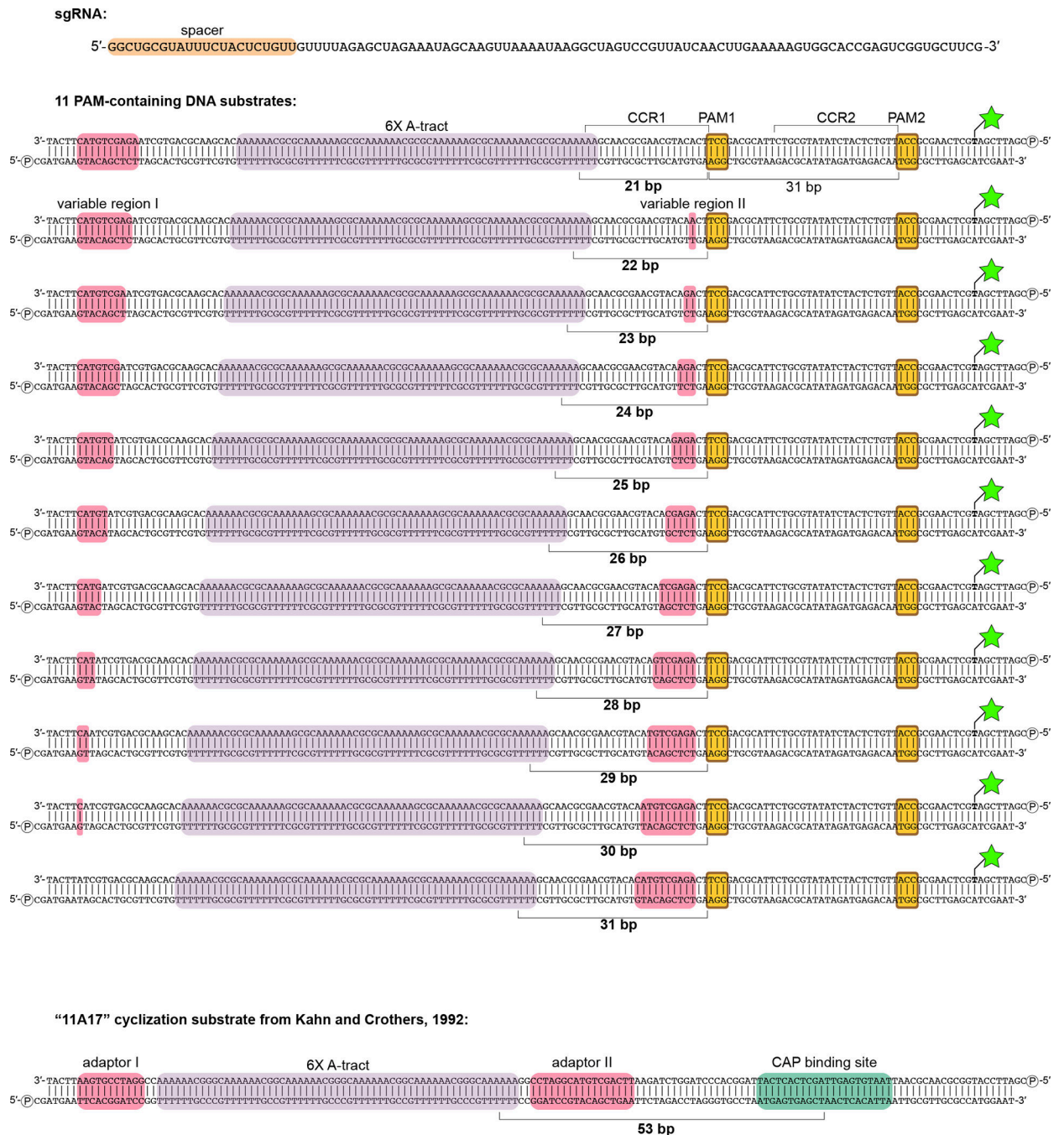
Extended Data Fig. 5. Nucleic acid sequences used in DNA cyclization experiments. Green star/bold T, fluorescein-conjugated dT; circled P, 5' phosphate; CCR, candidate complementarity region.
