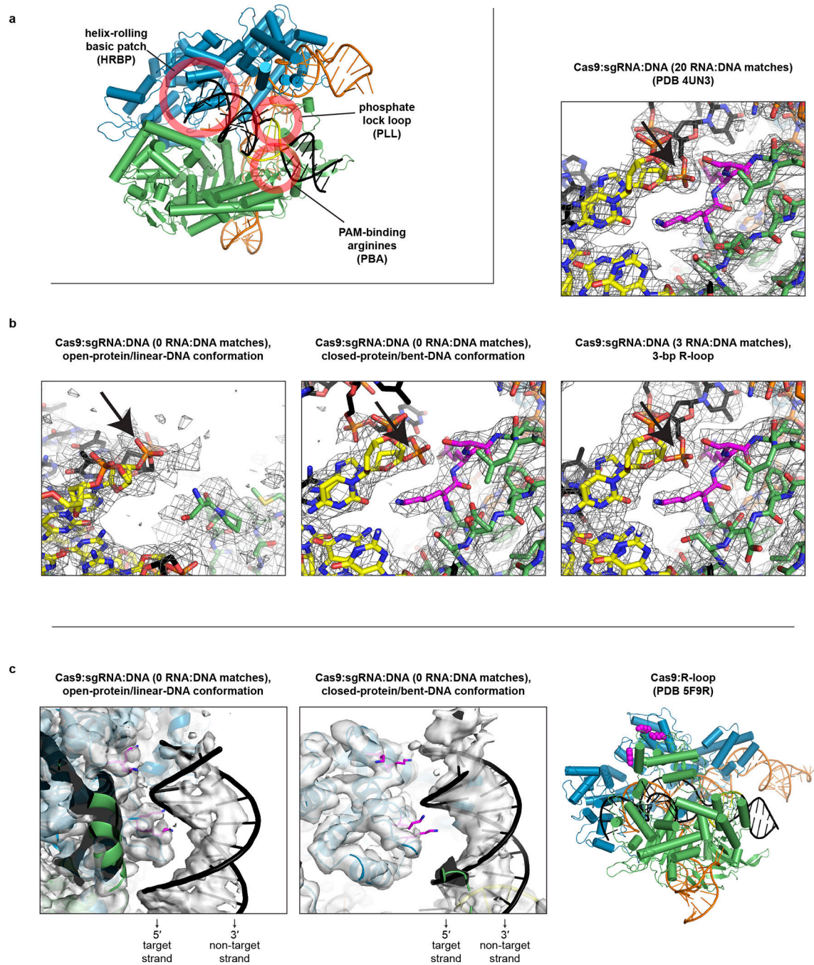
Extended Data Fig. 8. Structural features potentially relevant to Cas9-induced DNA bending. a. Location of each feature in the bent-DNA structure. Green, NUC lobe; blue, REC lobe; orange, guide RNA; black, DNA; yellow, PAM. b. Comparison of phosphate lock loop (magenta) in various structures, within sharpened cryo-EM maps (row of three, threshold 8\sigma ) or 2Fo-Fc map (upper right, threshold 1.5\sigma ). Black arrow indicates the eponymous
