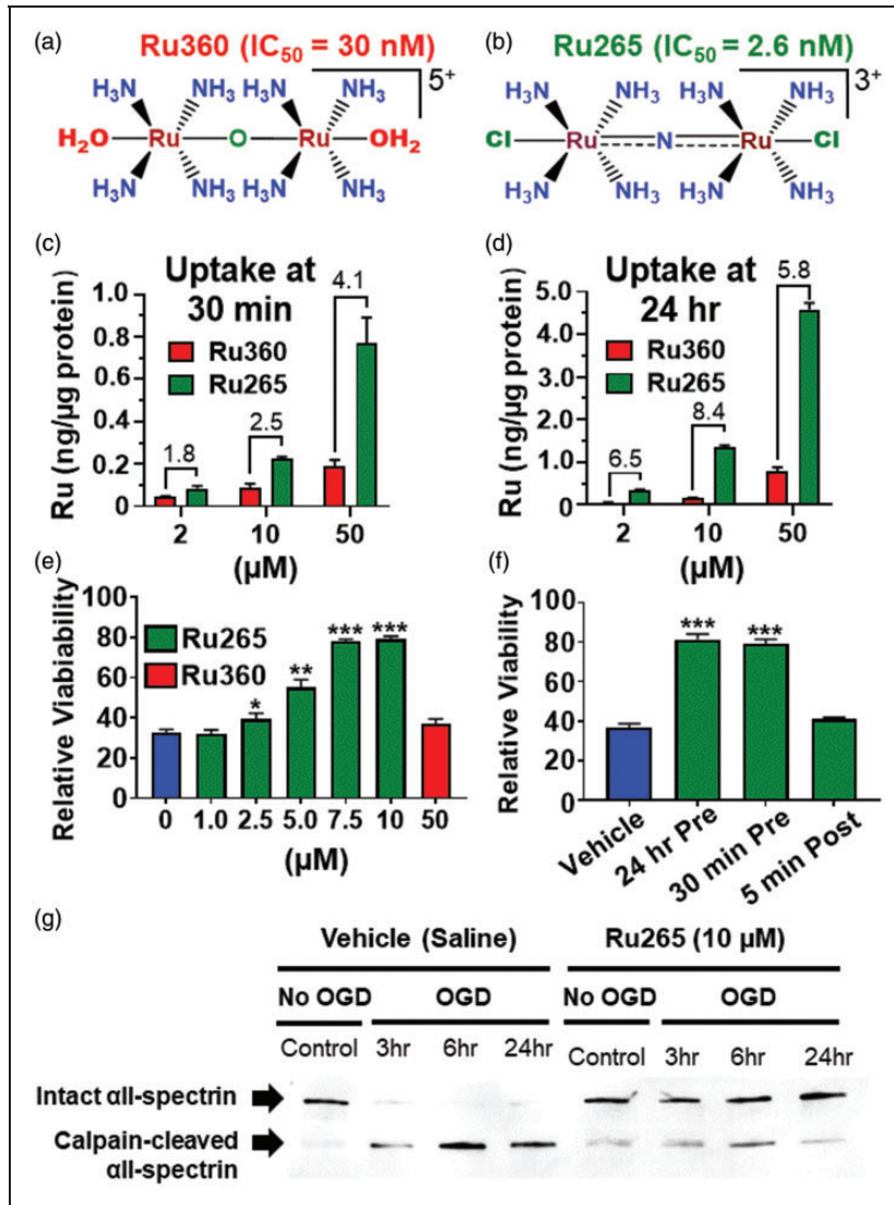
Figure 1. Chemical structures of Ru360 (a) and Ru265 (b). Ruthenium (Ru) concentrations in lysates of cortical neuron cultures 30 min and 24 h after treatment with Ru360 (2, 10 and 50 μM) and Ru265 (2, 10 and 50 μM; c and d). Comparisons of cell viability in cortical neuron cultures treated with Ru265 or Ru360 and subjected to lethal OGD (90 min, e). Cell viability in cortical neuron cultures treated with Ru265 before or immediately after OGD (f). Viability was assessed using a 3-(4,5-dimethylthiazol-2-yl)-2,5-diphenyl-tetrazolium bromide (MTT) assay 24 h after OGD. Values represent viability relative to control cortical cultures (no OGD). Bars show the mean ± SD of data from four separate experiments. * p < 0.05, ** p < 0.01 and *** p < 0.001 relative to vehicle (0 μM), Mann–Whitney U tests. Western blot showing calpain-mediated cleavage of the structural protein αII-spectrin in cortical neurons treated with vehicle or Ru265 and subjected to OGD (g).
