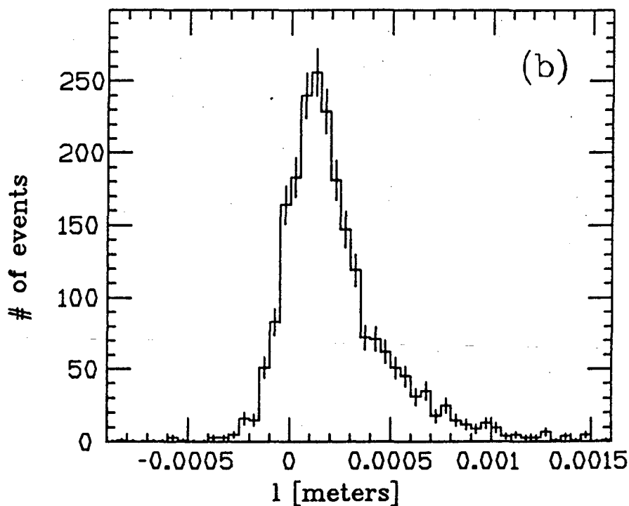
Figure 8.3 Decay length distribution (laboratory frame) of \tau \rightarrow 3\pi^{\pm}\nu events for (a) a \tau lifetime of c\tau = 0 , and (b) a \tau lifetime of c\tau = 0.0858 mm.
