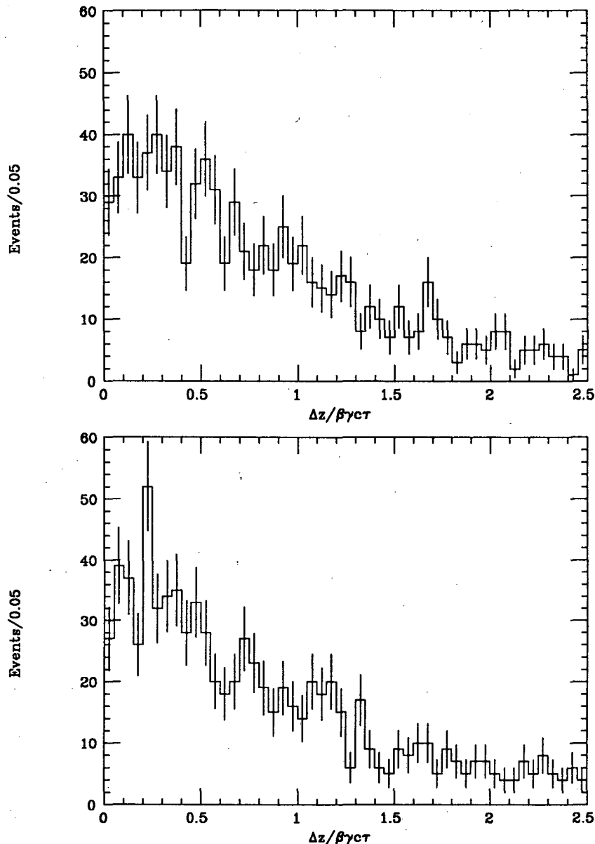
Figure 6.3 a&b The (smeared) decay path length distribution for C = +1 B , meson pairs; the upper plot is for opposite-sign lepton events, the lower for like-sign lepton events. This represents 30 \text{ fb}^{-1} of data, with x_s = 10 and \sigma = 0.25 \langle \Delta z \rangle .
