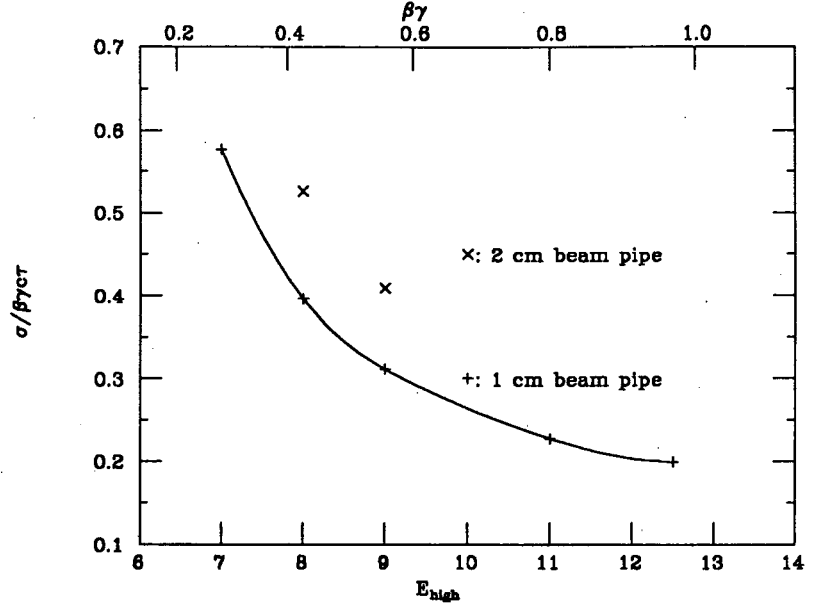
Figure 5.7 The resolution for measuring \Delta z , the distance between B decays, scaled by the mean distance between the decay ( \beta\gamma\tau ) as a function of boost and beampipe radius.
