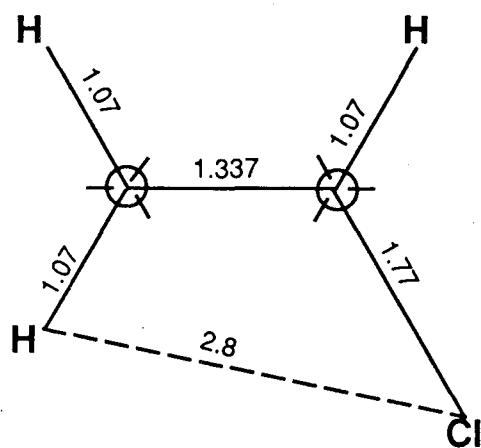
chloroethylene
