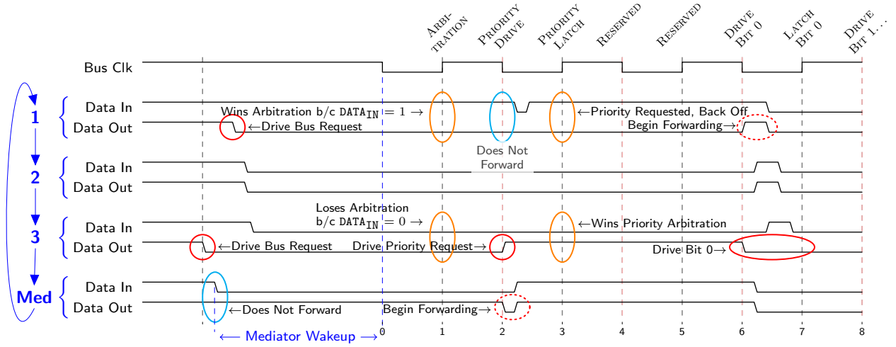
Figure 3.5: MBus arbitration. To begin a transaction, one or more nodes pull down on \text{DATA}_{\text{OUT}} . This shows node 1 and node 3 requesting the bus at nearly the same time (node 1 shortly after node 3). Node 1 initially wins arbitration, but node 3 uses the priority arbitration cycle to claim the bus. The propagation delay of the data line between nodes is exaggerated to show the shoot-through nature of MBus. Momentary glitches caused by nodes transitioning from driving to forwarding are resolved before the next rising clock edge.
