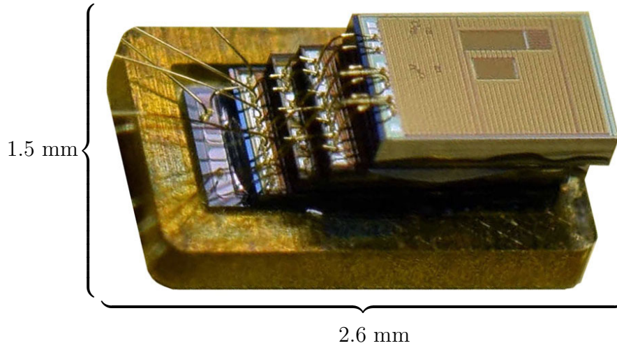
Figure 5.5: Temperature sensing system. A system designed as part of the Michigan Micro Mote project consisting of a 2\mu\text{Ah} battery, a 900 MHz near-field radio, an ARM Cortex M0 processor, and an ultra-low power temperature sensor, interconnected using MBus.
