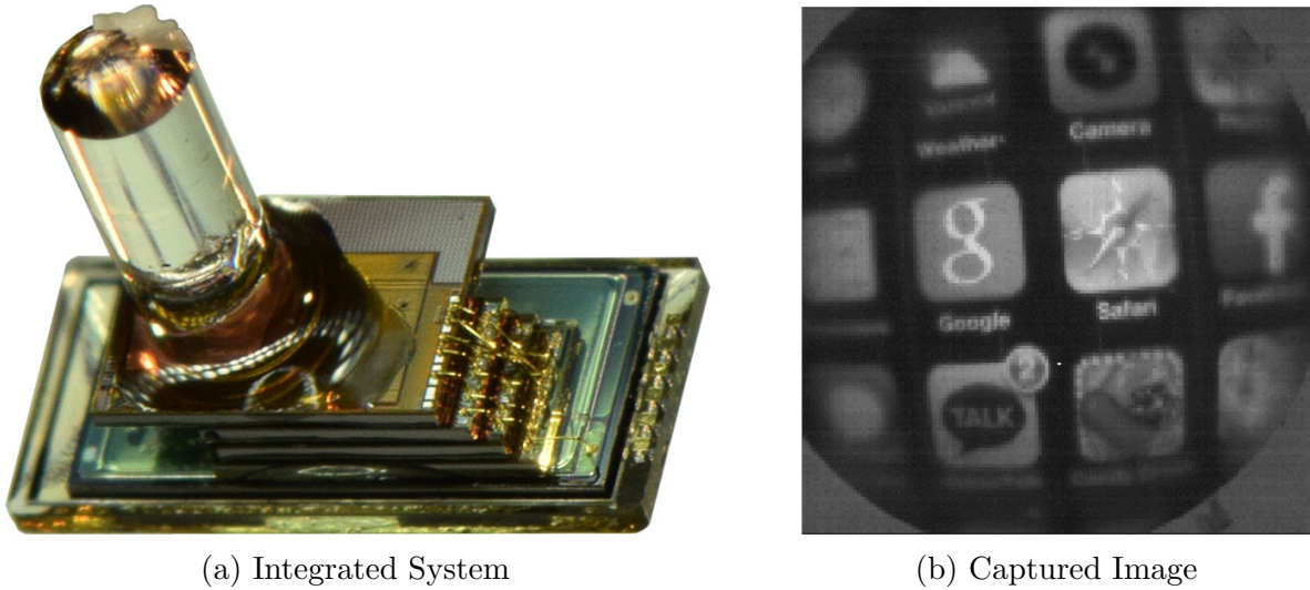
Figure 5.6: Motion detection and imaging system. (a) An imager made of a 900 MHz near-field radio, a 5 \mu AH battery, an ARM Cortex M0, and a 160 \times 160 pixel, 9-bit grayscale imager with ultra-low power motion detection all connected using MBus. (b) A full-resolution (28.8 kB) image that was transferred by MBus.
