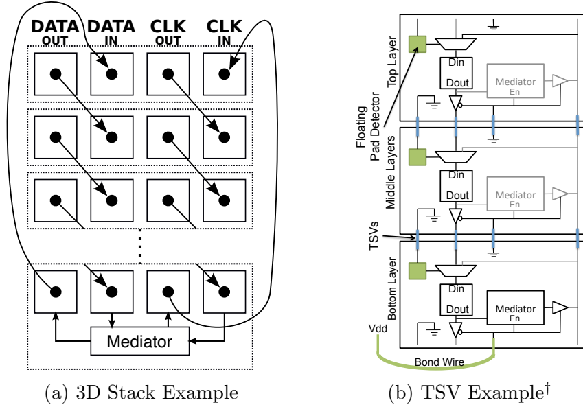
Figure 3.1: MBus topology. An MBus system consists of a mediator node and one or more member nodes connected in two “shoot-through” rings. The ring topology adapts to many system synthesis methods, such as stepped 3D-stacking with wirebonding (a) and TSVs (b).
