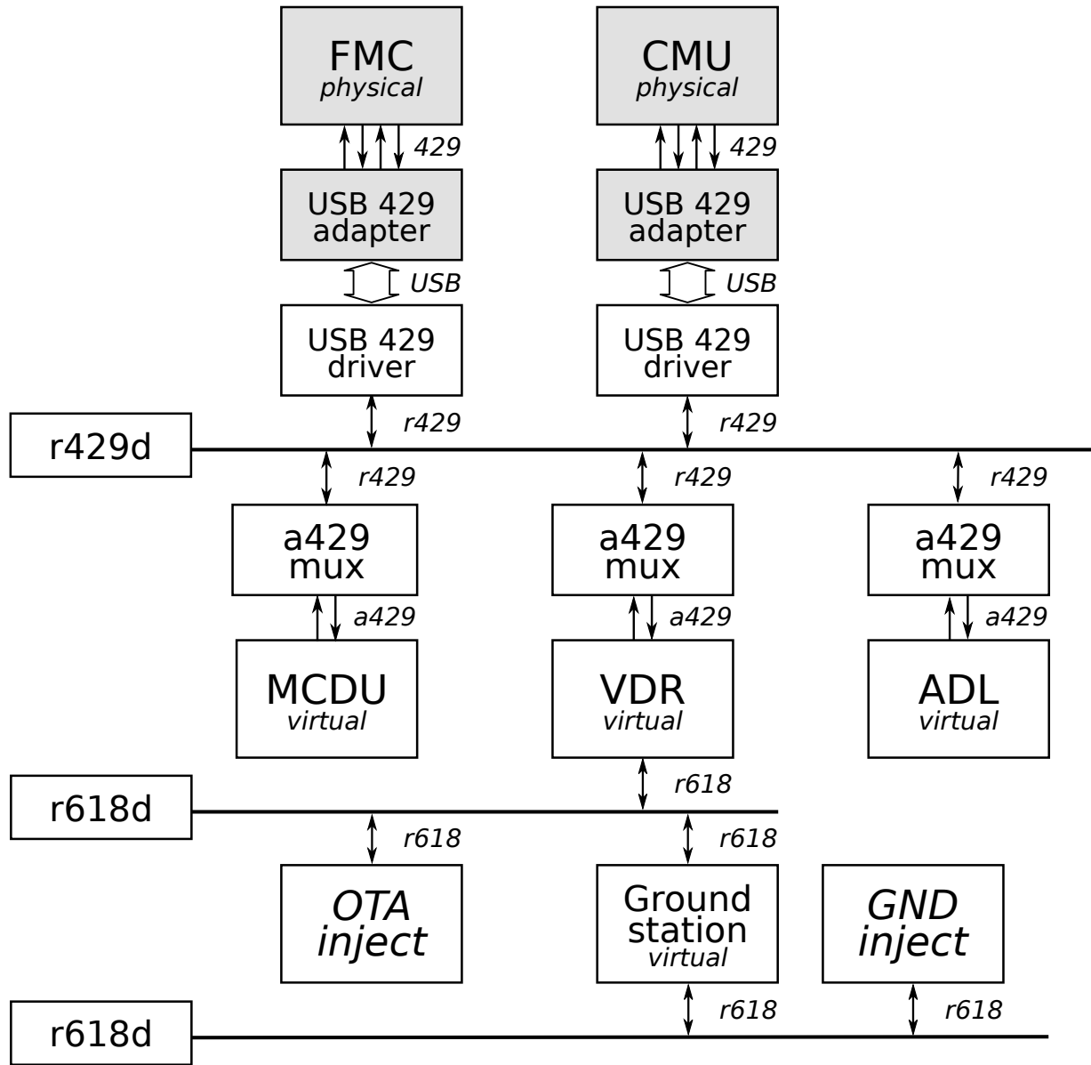
Figure 3.2: Portion of the Triton testbed.
