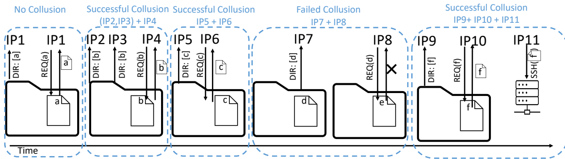
Figure 3.2. Identifying Colluding IP Addresses — We identified colluding IPs using the causal dependencies created by hourly-updated filenames. “DIR: [a]” is the return of a directory listing with the filename “a,” “REQ(a)” is the request of “a,” and “SSH(a)” is the extraction of SSH credentials from “a.”
