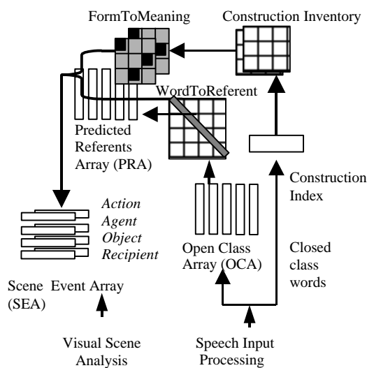
Figure 1. Structure-Mapping Architecture.
