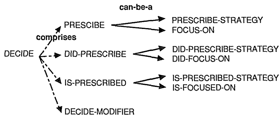
Figure 4.22: Type Hierarchy of DECIDE
