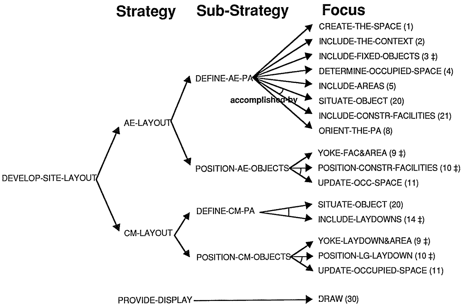
Figure 6.31: Skeletal Plan of the Temporal Strategy applied to AMI. The numbers in parentheses label the foci so that this skeletal plan can easily be compared to those of Figures 6.1, 6.2, 6.25, and 6.41. A focus with number labeled “‡” is similar to the one with corresponding number in the other figures, except for some small changes.
