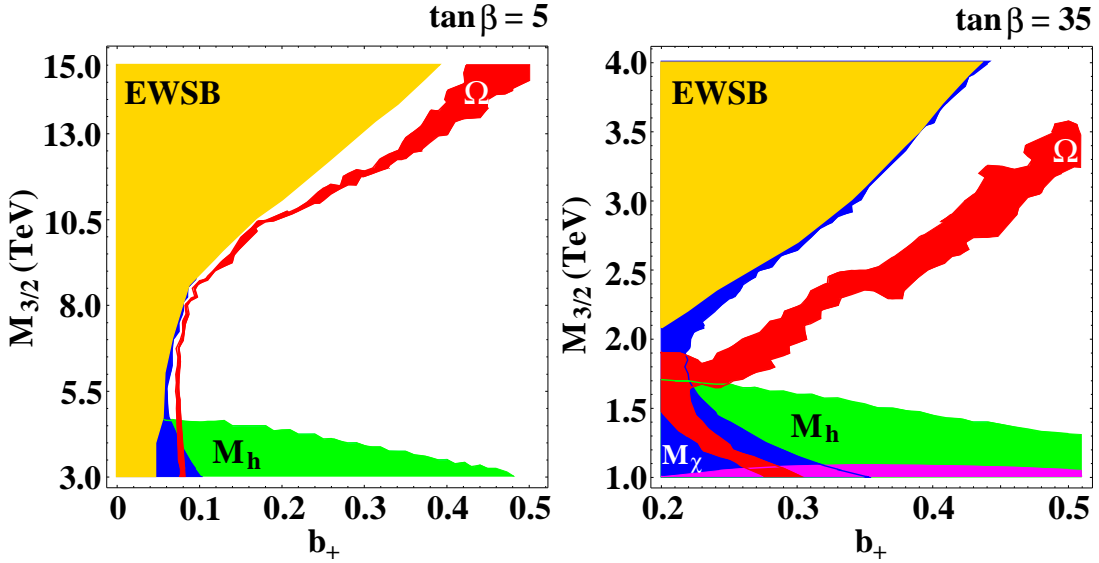
Figure 13: Constraints on the dilaton-dominated parameter space for \tan \beta = 5 (left) and \tan \beta = 35 (right) with \mu > 0 . Constraints on the (M_{3/2}, b_+) plane are given for \mu > 0 .
