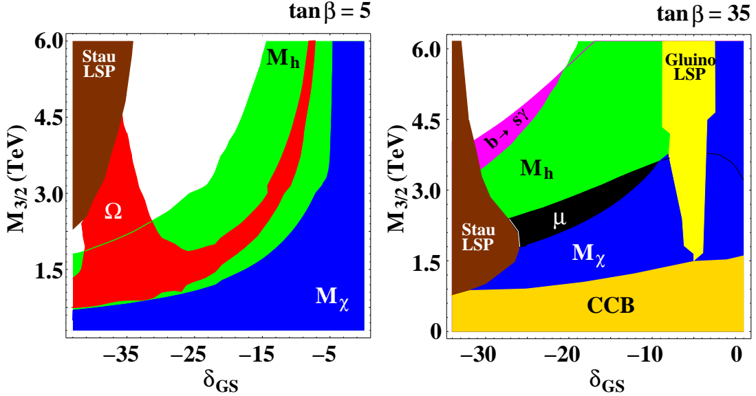
Figure 11: Constraints on the moduli-dominated parameter space for \tan\beta = 5 (left) and \tan\beta = 35 (right) with p = 0 and \langle \text{Re } t \rangle = 2.0 . Constraints on the (M_{3/2}, \delta_{GS}) plane are given for \mu > 0 . The dark shaded regions on the left have a stau LSP. The \tan\beta = 35 plot also has a region with a gluino LSP. For \tan\beta = 5 the region labeled “ \Omega ” has the cosmologically preferred relic density of neutralinos. No such region exists for the higher \tan\beta plot. In that case the exclusion contours are due to (from bottom right to upper left) CCB vacua, the chargino mass, too large SUSY contributions to (g_\mu - 2) , the Higgs mass limit and too large a b \rightarrow s\gamma rate.
