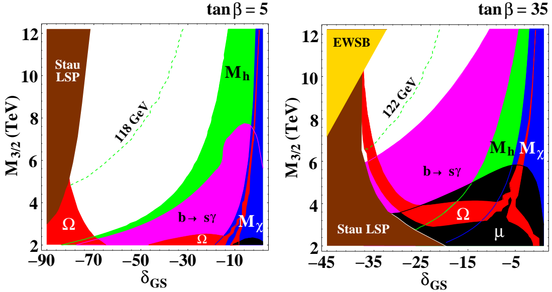
Figure 9: Constraints on the moduli-dominated parameter space for \tan\beta = 5 (left) and \tan\beta = 35 (right) with p = 0 and \langle \text{Re } t \rangle = 0.5 . Constraints on the (M_{3/2}, \delta_{GS}) plane are given for \mu > 0 . Shaded regions to the left are ruled out by improper EWSB or a stau LSP. The dark region in the lower right of the \tan\beta = 35 plot labeled “ \mu ” has too much supersymmetric contribution to (g_\mu - 2) . The strip labeled “ \Omega ” has the cosmologically preferred neutralino relic density. Dashed contours of m_h = 118 GeV (left) and m_h = 122 GeV (right) are also given.
