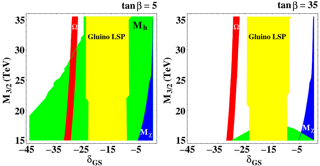
Figure 10: Constraints on the moduli-dominated parameter space for \tan\beta = 5 (left) and \tan\beta = 35 (right) with p = 0 and \langle \text{Re } t \rangle = 1.23 . Constraints on the (M_{3/2}, \delta_{GS}) plane are given for \mu > 0 . The lightly shaded region in the center gives a gluino LSP. The thin strip with acceptable thermal neutralino relic density is labeled “ \Omega .” Note the change in scale from Figure 9.
