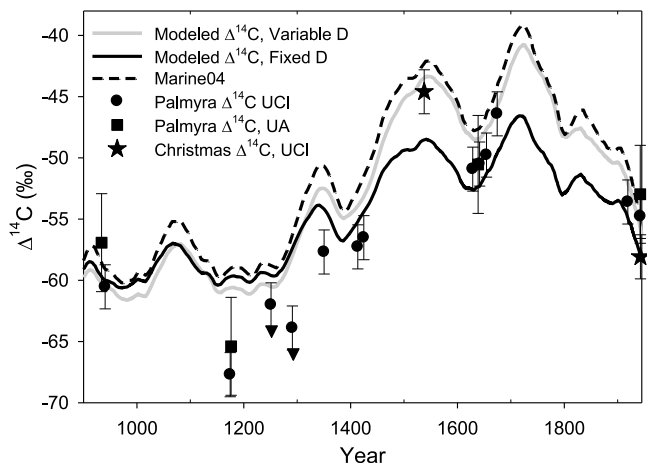
Figure 6. Comparison of Palmyra mixed layer model \Delta^{14}\text{C} with measured Palmyra and Christmas coral \Delta^{14}\text{C} over the last millennium. Palmyra mixed layer model output for fixed (solid black line) and variable (solid gray line) \Delta^{14}\text{C} values for deep water boxes are plotted with Marine04 [Hughen et al. , 2004] (dashed line) and average measured coral \Delta^{14}\text{C} values for each modern and fossil coral segment. Error bars represent the analytical errors of \pm 1.8\% for data generated at UCI, or \pm 4.0\% for data generated at UA. The 13th century fossil coral \Delta^{14}\text{C} are plotted as maximum values, as secondary carbonates with higher \Delta^{14}\text{C} contaminate this coral (downward arrows reflect the fact that the primary coral \Delta^{14}\text{C} are likely lower than the \Delta^{14}\text{C} values measured).
