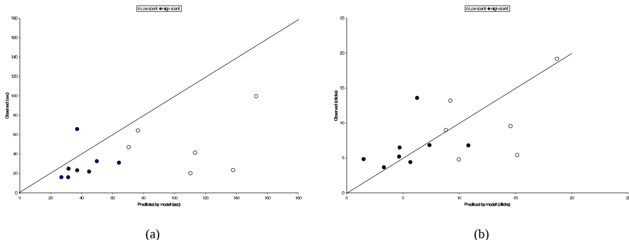
Figure 3: Model results (x axis) against data (y axis): (a) search times; (b) clicks.
