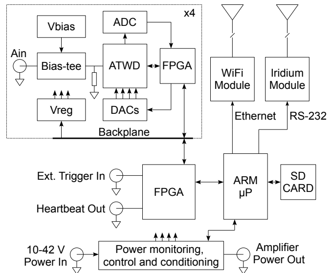
Fig. 10: Simplified block diagram of the ARIANNA system hardware.
