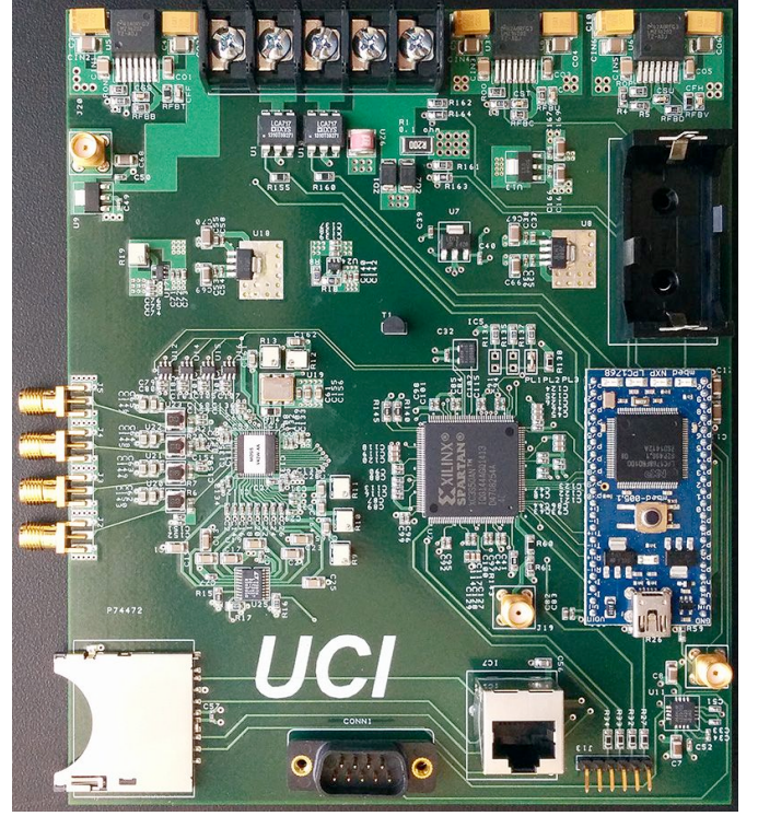
Fig. 27: The next-generation ARIANNA single-board data acquisition system. It includes one four-channel SST chip (left of center), improved power management and protection, on-board temperature monitoring, and has significantly-lower cost and calibration requirements. Average power consumption has been reduced from ~5.8W to ~1.7W.
