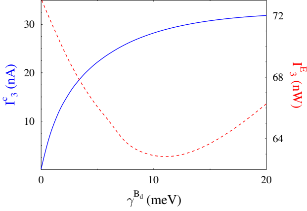
FIG. 2: (Color online) Molecular pump (Fig. 1a). Shown are the charge ( I_3^c , Eq.(9) - solid line, blue), and energy ( I_3^E , Eq.(10) - dashed line, red) fluxes on the right interface as functions of dephasing rate \gamma^{B_d} , Eq.(15). See text for parameters.
