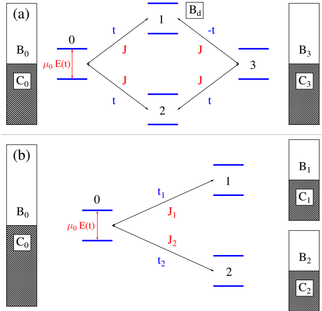
FIG. 1: (Color online) A sketch of the models for coherently controlled charge-energy (a) pump and (b) switch.
