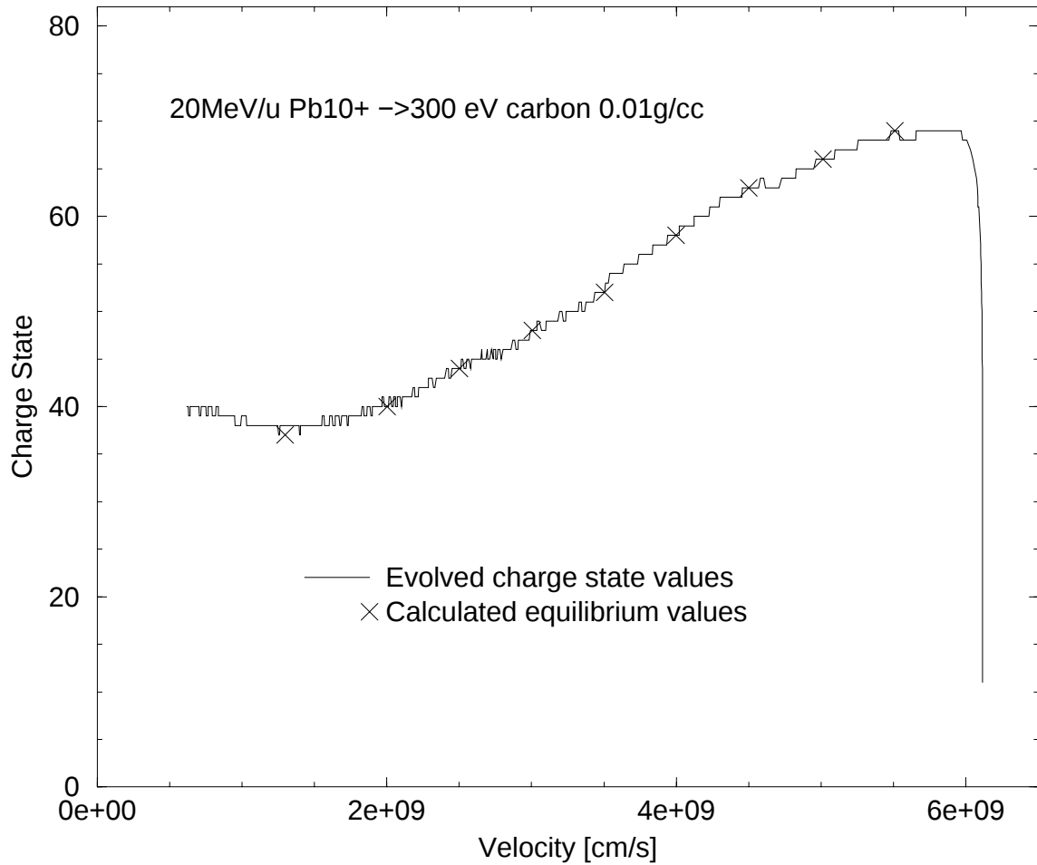
Figure 7.10: Charge states for a 20MeV/u lead projectile penetrating a carbon plasma of average charge 5.9+ at 0.01\text{gcm}^{-3}
