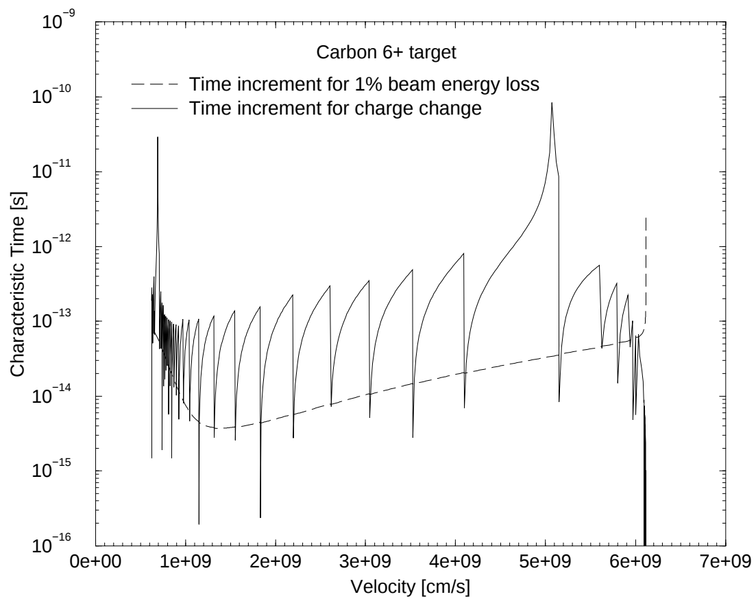
Figure 7.7: Charge change and energy deposition time increments for a 20\text{MeV}/u lead projectile penetrating a carbon plasma of average charge 6+ at 0.01\text{gcm}^{-3}
