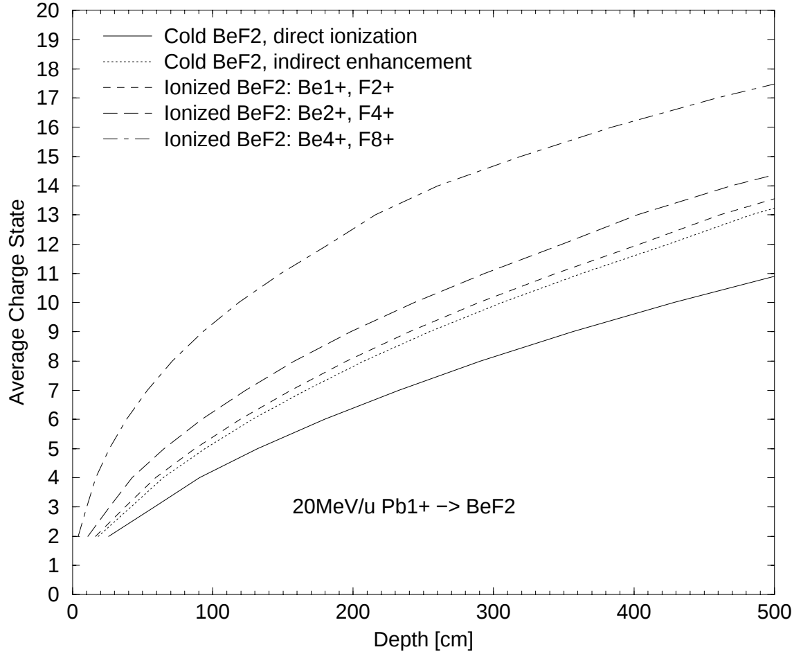
Figure 7.2: Various charge evolution calculations for a 20MeV/ u Pb beam penetrating HIF chamber plasma of 5 \times 10^{13} \text{cm}^{-3} BeF 2 ; dotted line shows results using cross sections multiplied by 1.4 and dashed line shows case of ionized BeF 2 (see text)
