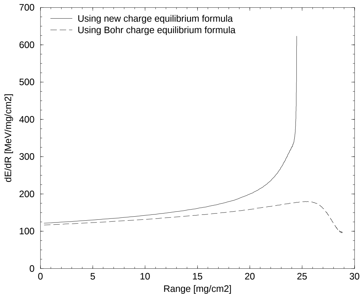
Figure 7.26: Energy deposition profiles for 20MeV/ u Pb penetrating a carbon plasma with \rho = 0.1\text{gcm}^{-3} at 300eV using both the new charge equilibrium fit and the cold matter fit
