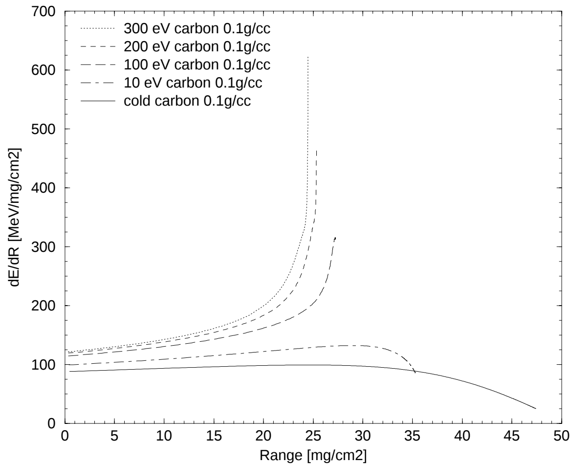
Figure 7.25: Energy deposition profiles for 20MeV/ u Pb penetrating a carbon plasma with \rho = 0.1\text{gcm}^{-3} at several temperatures
