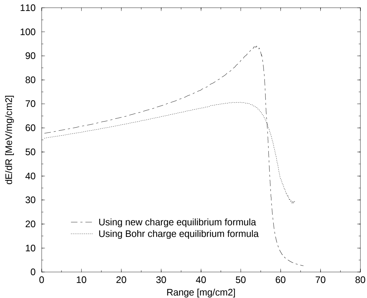
Figure 7.24: Energy deposition profiles for 20MeV/ u Pb penetrating a dense gold plasma with \rho = 1\text{gcm}^{-3} at 300eV using old and new charge equilibrium models
