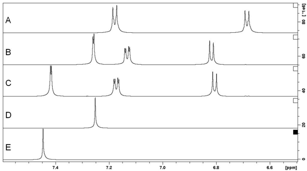
Figure 4.8. 1D ^1\text{H} NMR spectra of (A) tert -octylphenol, (B) tert -monochlorooctylphenol, (C) tert -dichlorooctylphenol, (D) tert -monobromooctylphenol and (E) tert -dibromooctylphenol.
