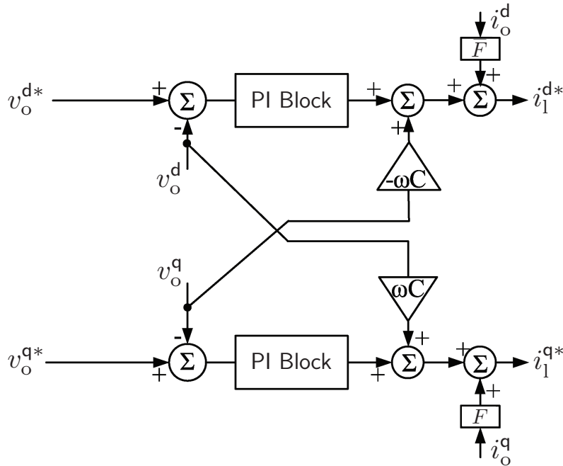
Figure 2.12: Typical device-level voltage controller block diagram.
