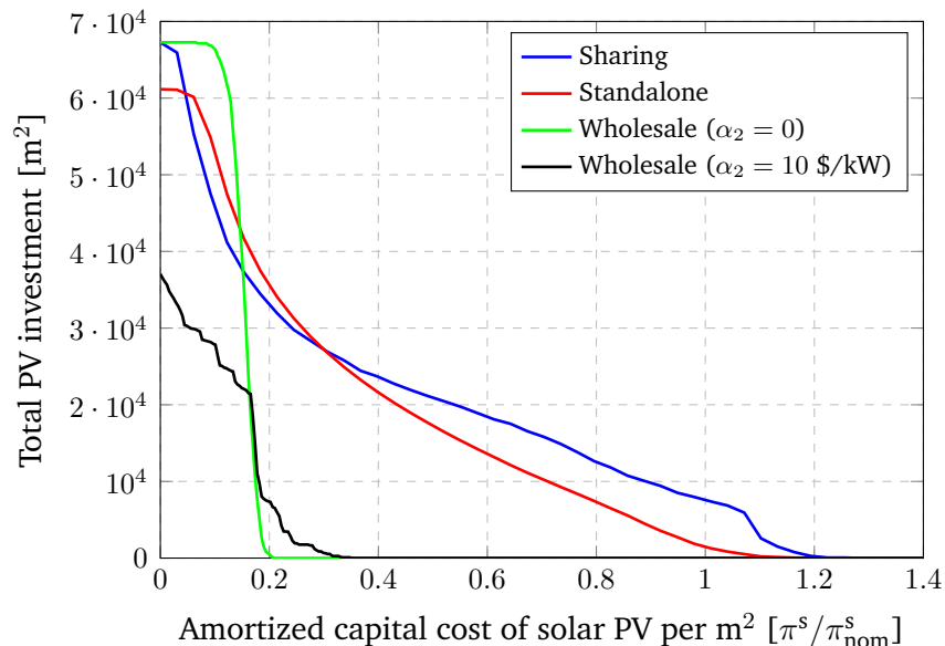
Figure 3.12: Total PV investment among different models when varying the amortized capital cost of PV \pi^s in Case 3. The x -axis is the ratio of amortized cost against the nominal solar PV cost \pi_{\text{nom}}^s = 0.0047 \$/\text{m}^2 (per time slot).
