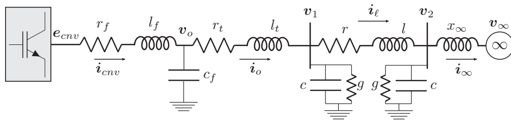
Figure 2.22: One-line diagram for study cases.
