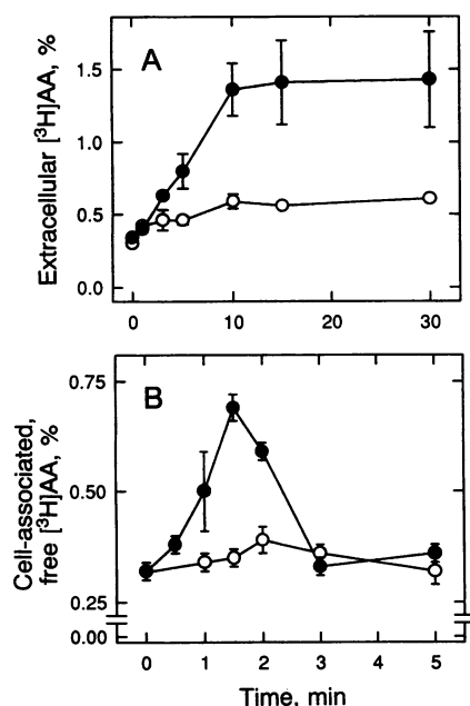
FIG. 2. AA release in activated P388D 1 cells. (A) Time course of the extracellular release of [^3\text{H}]\text{AA} . (B) Time course of the accumulation of cell-associated, free [^3\text{H}]\text{AA} . LPS-primed cells, prelabeled with [^3\text{H}]\text{AA} for 20 h, were incubated with (●) or without (○) PAF (20 nM). Radioactivity released into the medium (A) or cell-associated [^3\text{H}]\text{AA} (B) was measured at the indicated time points. Data in A represent the means \pm SEM of three different experiments and are expressed as the percentage of radioactivity released into the incubation medium compared to the total cellular radioactivity. Data in B are presented as means \pm SEM from one experiment with triplicate determinations and are expressed as the percentage of radioactivity in free [^3\text{H}]\text{AA} in cells compared to the total cellular radioactivity.
