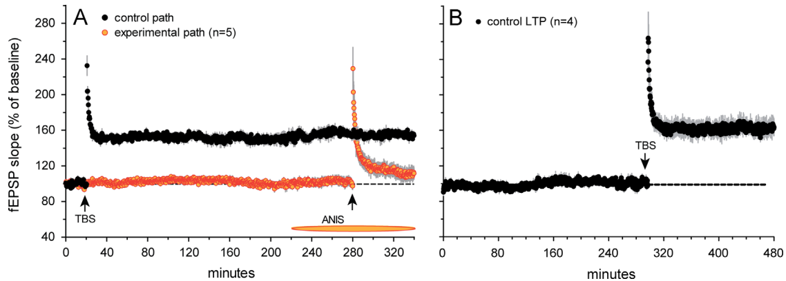
Fig. 3 – A protein synthesis inhibition blocks LTP in ‘mature’ slices. (A) Stable baseline recordings of Schaffer-commissural fEPSPs were collected from CA1b stratum radiatum for 4.5 h before applying ANIS to the slice bath 30 min prior to TBS (6 h after slice preparation). Under these conditions, TBS of the ‘experimental’ path induced an initial potentiation but the fEPSP slope gradually returned to baseline levels over a 1 h recording period. LTP induced 4.5 h earlier in a separate population of axons (‘control path’) was unaffected by the inhibitor. (B) In a separate set of slices, baseline recordings were collected for 4.5 prior to delivery of TBS (6 h after cutting) in the absence of the inhibitor. Robust LTP was obtained and remained stable during the 3 h post-TBS recording session.
