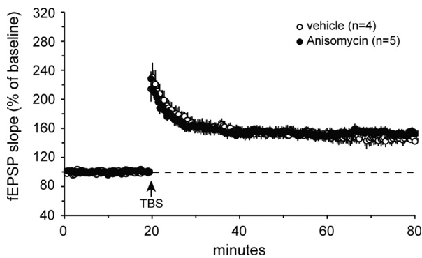
Fig. 4 – Incubation with anisomycin during slice preparation and through delivery of TBS fails to block LTP. Adult rat hippocampal slices were sectioned in the presence of 40 \mu\text{M} anisomycin and then continuously treated with inhibitor or vehicle (0.01% DMSO) in ACSF for the following 2.5 h. After 2 h of incubation and 20 min of stable baseline recording, TBS was applied to Schaffer/commissural afferents of CA1b stratum radiatum where fEPSPs were recorded. As shown, potentiation was robust, stable, and of comparable magnitude in slices incubated in anisomycin or vehicle. Note that the inhibitor incubation time for this study was much longer than that employed in the studies described in Fig. 3A.
