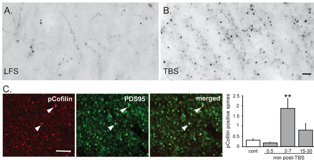
Fig. 1 – Theta burst stimulation (TBS) promotes actin polymerization and cofilin phosphorylation in adult hippocampal slices. Images were collected from proximal CA1b stratum radiatum following stimulation of Schaffer/commissural afferents. (A,B) In situ phalloidin labeling in slices that received (A) baseline low-frequency stimulation (LFS) or (B) TBS illustrates the increase in F-actin enriched spines (dark puncta) achieved with theta stimulation. (C) Deconvolved epifluorescence images show immunolabeling for phosphorylated (p) Cofilin, and excitatory synapse scaffold protein PSD95, and the merged image of the two for the same field; arrowheads indicate double-labeled synapses. Cofilin is downstream effector of RhoA: phosphorylation inactivates this F-actin severing protein thus allowing actin polymers to survive and elongate. Quantification of spine labeling (bar graph, right) shows that TBS transiently increases numbers of pCofilin + enriched contacts indicating transient cofilin inactivation (mean ± SEM values for 8–9 slices/group; ** p=0.008 vs controls). Scale bars 5 \mu\text{m} (in B for A and B). Modified from Baudry et al. (2012) and Chen et al. (2007).
