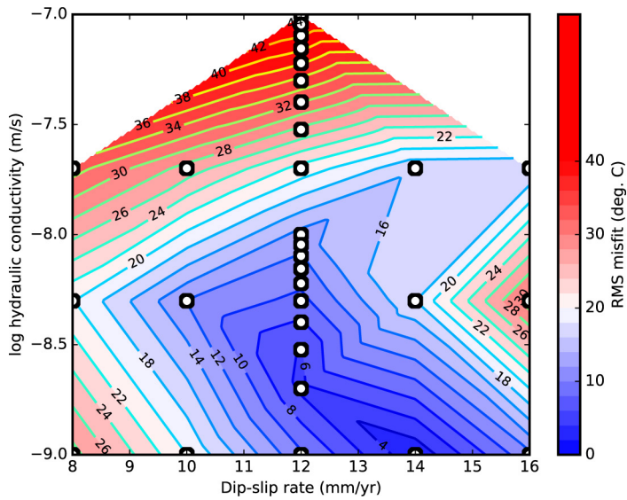
Extended Data Figure 5 | Fit of FEFLOW models to observations at DFDP-2B by varying parameters. Variable parameters are the (uniform) hanging-wall permeability to 3 km below sea level, and the dip-slip rate on the Alpine Fault. White dots indicate the parameter combinations of specific models. RMS, root mean square.
