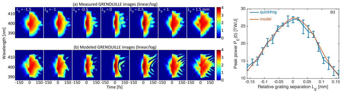
Fig. 15. (a) Measured GRENOUILLE images for multiple L_{g'} = L_g - L_{opt} , where L_{opt} is the optimized grating distance. The left side of each image is shown in linear scale and the right side in log scale. The linear scale images were normalized into the peak of the log scale image. For each L_g , 10 shots were acquired, and binned by 3x3 pixels to gain dynamic range. (b) Fit GRENOUILLE images based on the 12th order polynomial \phi^{in} in log and linear scales. (c) The peak power P_E(0) comparison between Quickfrog analysis and the modeled laser pulse. The errorbar for Quickfrog analysis shows the minimum and maximum of 10 shots acquired for each L_{g'} .
