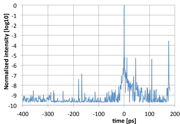
Fig. 10. Sub-nanosecond pulse structure measured by SEQUOIA with 1 ps step and 3-shot averaging at each step. The input energy was about 0.2 mJ.
