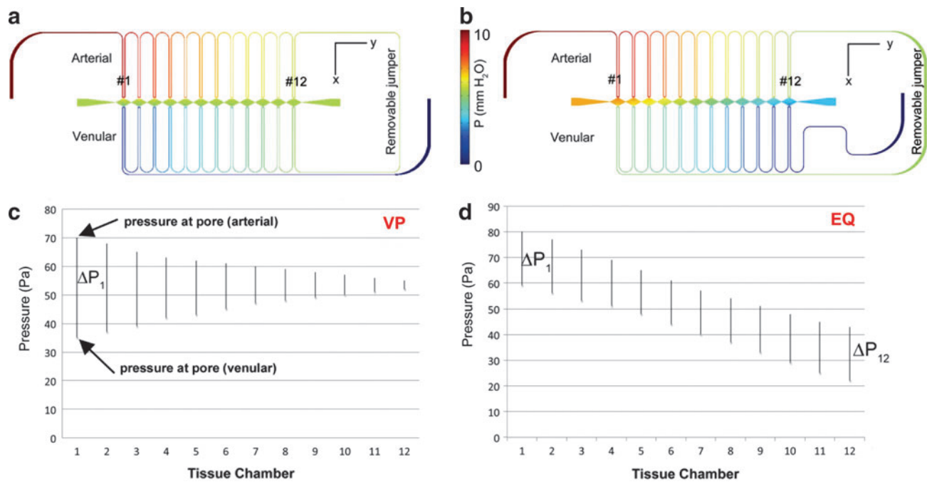
FIG. 2. Finite element simulations demonstrate the ability to control the pressure distribution ( a , b ) and subsequent interstitial flow distribution within the device. In the first design the transverse pressure gradient across the microtissue chamber is variable (VP), or ( \Delta P_1 > \Delta P_{12} ) while the mean pressure is constant ( c ). The alternate design creates equal (EQ) pressure gradients across the tissue microchambers ( \Delta P_1 = \Delta P_{12} ), although the mean pressure of the chambers decreases as chamber number increases ( d ). Color images available online at www.liebertpub.com/tec
