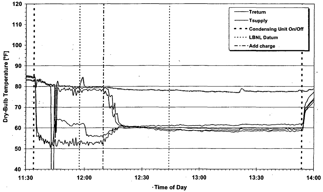
Figure A7c. Plenum temperature variations – Site 3.
