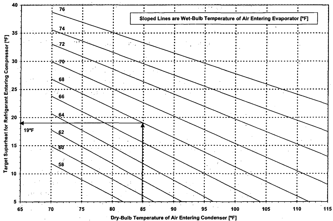
Figure 1. Refrigerant superheat charging chart.
