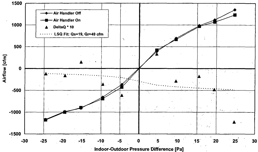
Figure A3. Sample DeltaQ test results.
