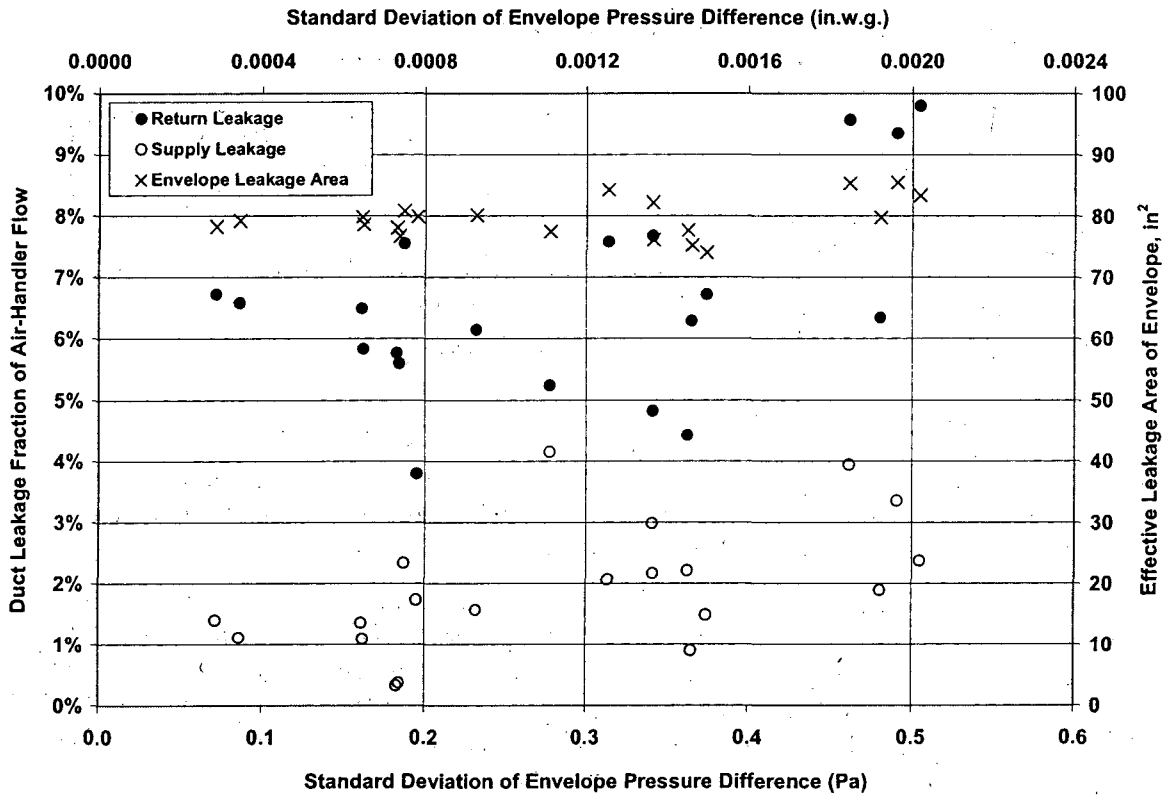
Figure A1. LBNL DeltaQ repeatability test results.
