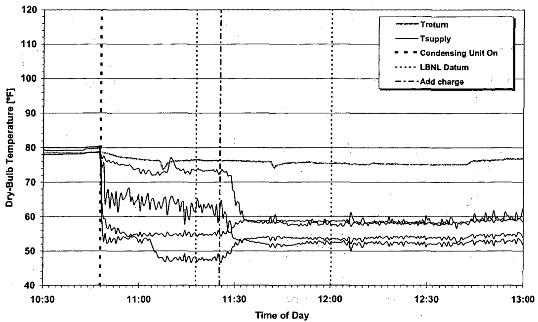
Figure A7b. Plenum temperature variations – Site 2.
