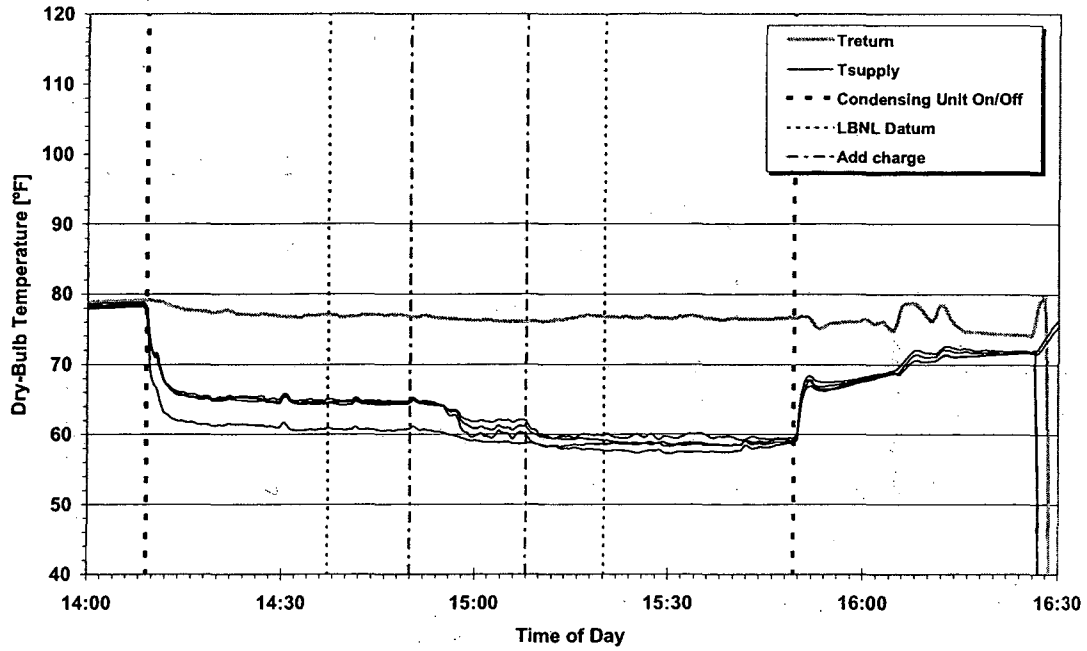
Figure A7a. Plenum temperature variations – Site 1.
