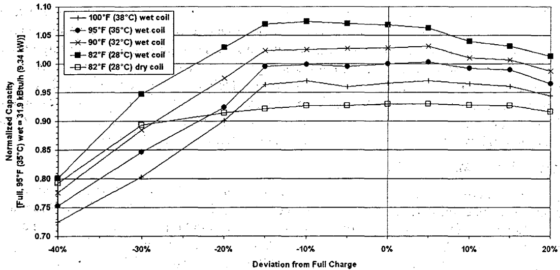
Figure A15. Total capacity variation – TXV (Farzad and O’Neal 1989).
