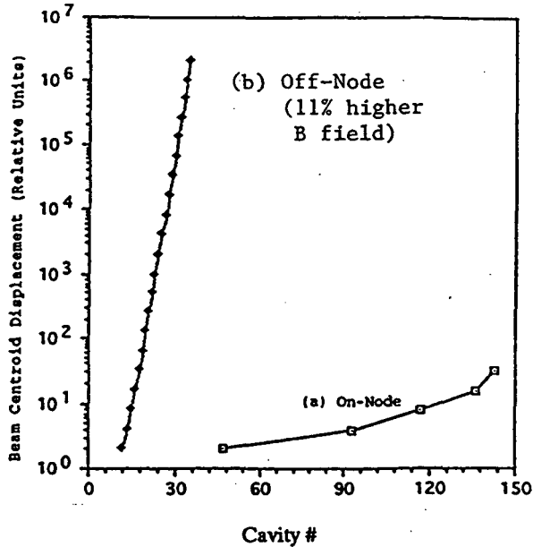
Fig. 3 Effect of the 'betatron-node' scheme on the BBU growth at 14 GHz.
