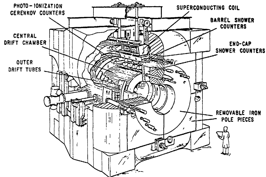
HIGH RESOLUTION SPECTROMETER ARGONNE - INDIANA - LBL - MICHIGAN - PURDUE - S.L.C
