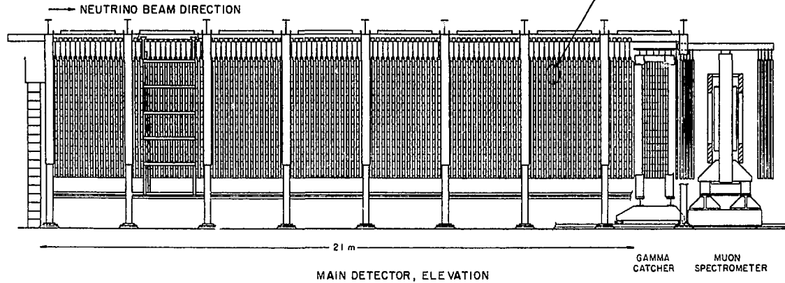
MAIN DETECTOR, ELEVATION
