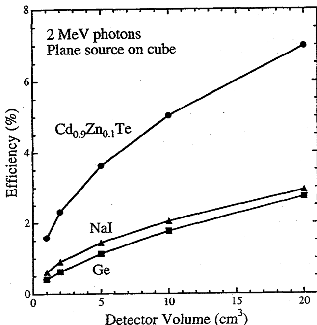
Figure 3. Calculated photopeak efficiencies of CdZnTe, Ge and NaI as a function of detector volume for 2 MeV photons.
