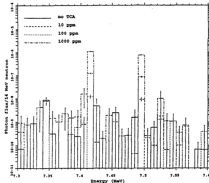
Figure 5. Effect of TCA concentration in water on the photon spectrum in the detector volume. Medium is made of sand (1.9 g/cc) and water (0.3 g/cc).
