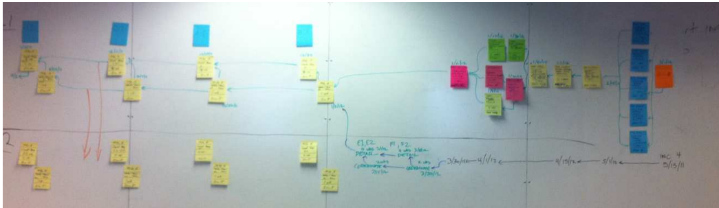
Figure 9: Pull Schedule for BIM Coordination (Source: Eric Osterling, Unger Constr.)
