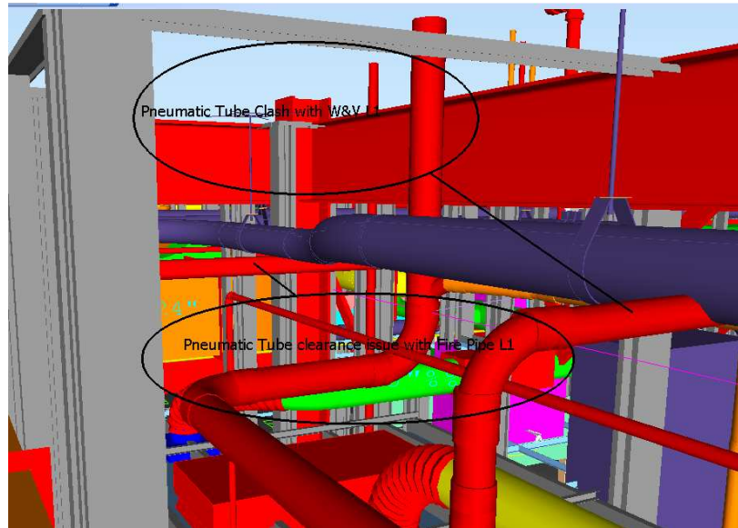
Figure 2: Hard Clash between Pneumatic Tube (purple) and Waste and Vent (W&V, red), and Soft Clash between Pneumatic Tube (purple) and Fire Pipe (red) (Source: Eric Osterling, Unger Construction)
