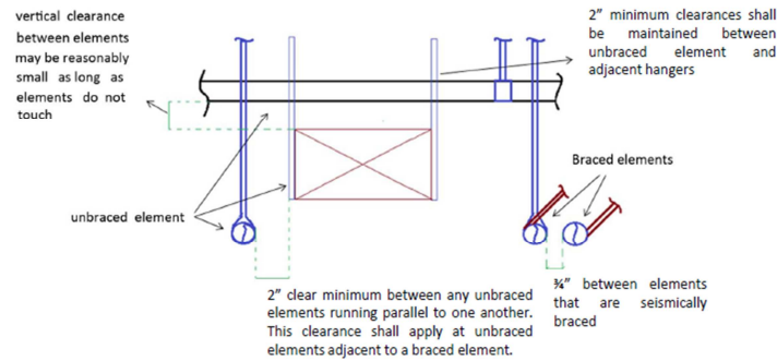
Figure 4: Component clearances (Source: Eric Osterling, Unger Construction)
