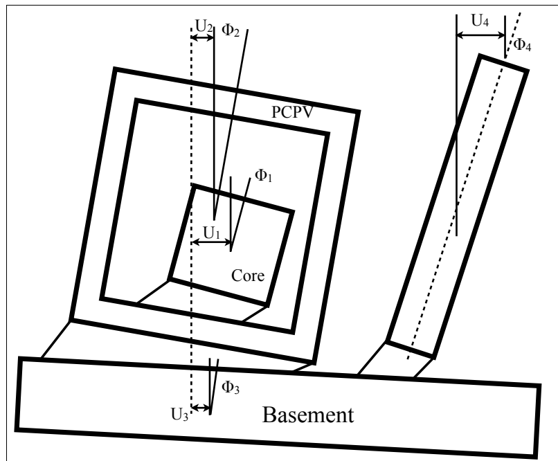
Figure 6.2: An 8 degree-of-freedom model of a nuclear power plant (taken from [27]).
