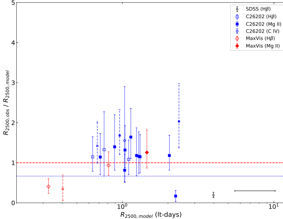
Figure 20. Ratio R_{obs}/R_{model} of the observed disk size to the predicted disk size vs. the thin disk model prediction. The symbols have the same meaning as Figure 19. The red dashed line is drawn at R_{obs}/R_{model} = 1 where the observed disk size equals the predicted disk size from the model using X = 5.04 . The blue dotted line is drawn at R_{obs}/R_{model} = 0.67 where the observed disk size equals the predicted disk size with X = 3.36 . The uncertainty of the predicted accretion disk is shown as the black errorbar in the bottom right corner, considering that the uncertainty of the black hole mass is about 0.4 dex.
