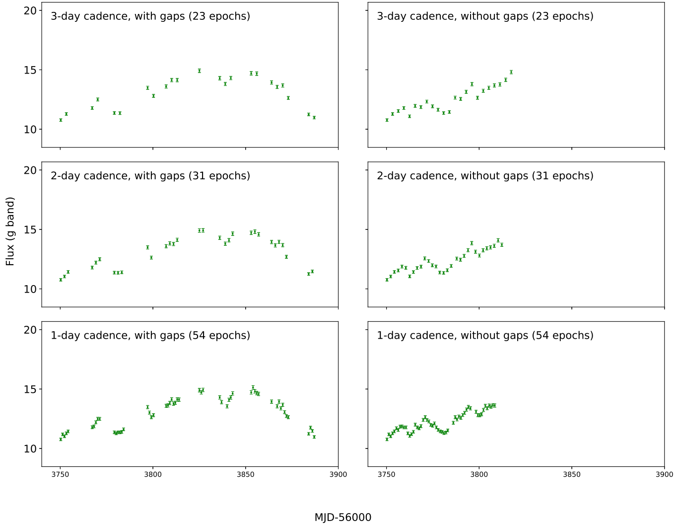
Figure 23. Simulated g -band lightcurves for one observational season for quasars in the LSST DDFs. The fluxes are in arbitrary units. The upper, middle and lower row show the lightcurve from a 3-day, 2-day and 1-day cadence from OpSim, respectively. The left column shows the lightcurves with gaps, while the right column shows the lightcurves where gaps are removed. The lightcurves with the 3-day, 2-day and 1-day cadence have about 23, 31 and 54 epochs in one observational season, respectively.
