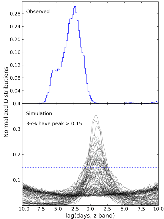
Figure 21. (upper panel) Probability distribution of the time lags in the z band from the observed lightcurves of DES J063227.29–583915.00 from JAVELIN. (lower panel) z -band lag distributions from 80 realizations of the simulated lightcurves of DES J063227.29–583915.00 with an input time lag of 1 day. The red dashed line shows the position of the input time lag. The blue dotted line shows the position where the probability density equals 0.15. Only 36% of the realizations show significant peaks with the peak probability density larger than 0.15.
