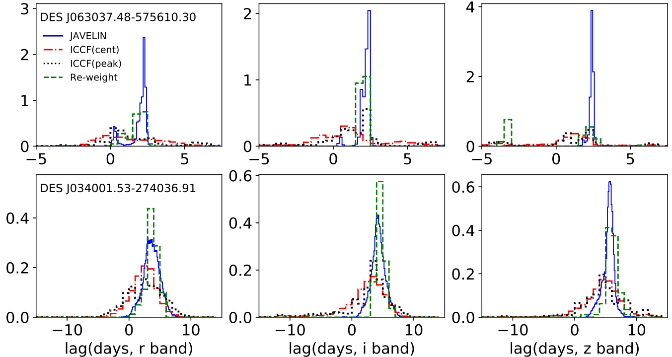
Figure 16. Probability distribution of time lags in the r , i , z band relative to g band for DES J063037.48–575610.30 (upper row) and DES J034001.53–274036.91 (lower row). The blue solid, red dash-dotted and black dotted lines represent the results from JAVELIN, the ICCF center distribution and the ICCF peak distribution, respectively. The green dashed line represents the distribution of the median JAVELIN lags from fitting the re-weighted lightcurves.
