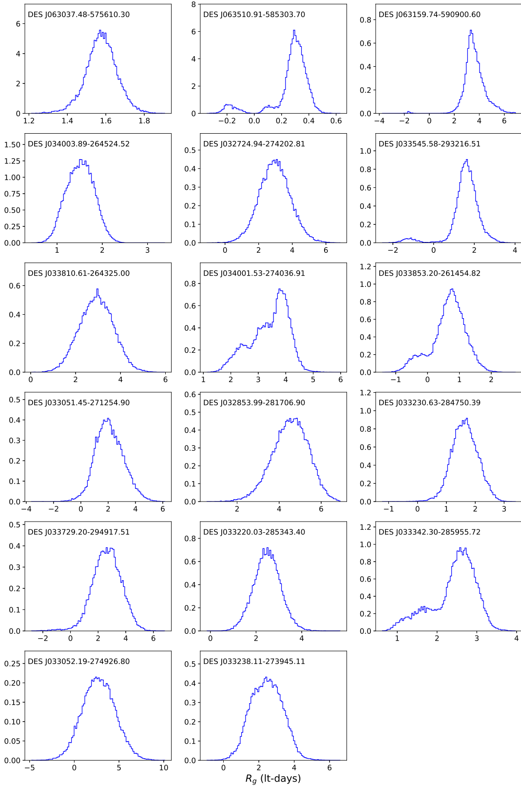
Figure 9. Probability distributions for the observed frame g -band accretion disk sizes from the JAVELIN Thin Disk model for quasars without flags in the main sample. Each panel shows the result for one object.
