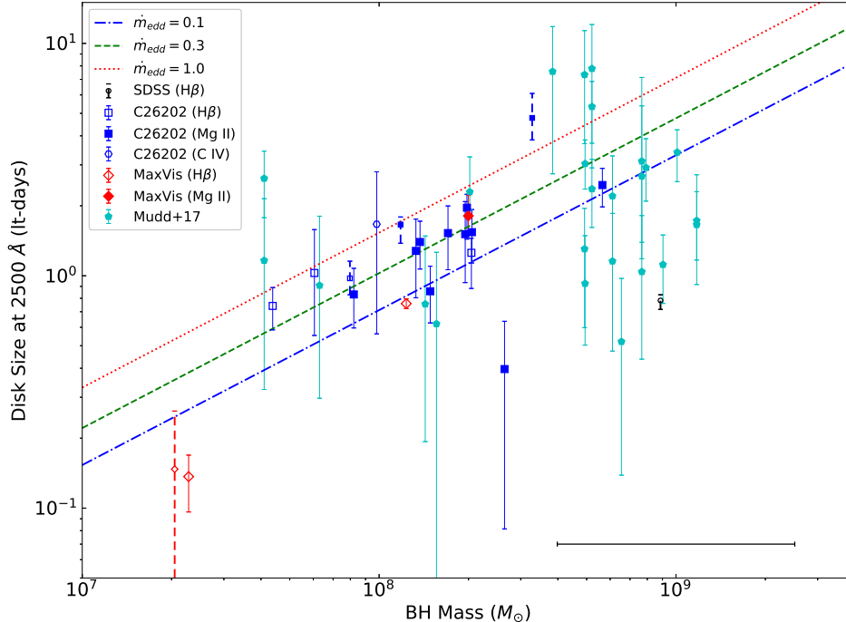
Figure 19. Accretion disk size at rest frame 2500 Å as a function of black hole mass. The blue dash-dotted, green dashed and red dotted lines represent the prediction of the thin disk model for Eddington ratios of 0.1, 0.3 and 1.0, respectively. The red diamonds, blue squares, black circles and cyan pentagons represent the results from the MaxVis field, the C26202 field, the SDSS fields and Mudd et al. (2018), with errorbars for the 1\sigma uncertainties. For the objects from this work, the smaller markers with dashed errorbars represent the flagged objects, while the larger markers with solid errorbars represent the objects with flag = 0 (the most secure results). The open hexagons represent black hole masses measured from C IV. Other open markers represent black hole masses measured from Mg II, while the filled markers represent black hole masses measured from H \beta . The typical uncertainty of the black hole mass is about 0.4 dex, shown as the black errorbar in the bottom right corner.
