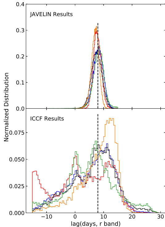
Figure 15. Probability distribution of r -band time lags relative to g -band from fitting the simulated DRW lightcurves of DES J032801.84–273815.72 with JAVELIN (upper panel) and ICCF (lower panel). The histograms with different colors in each panel represent the JAVELIN or ICCF results for different realizations of the DRW lightcurves. The black dashed line in each panel represents the position of the 8-day input time lag.
