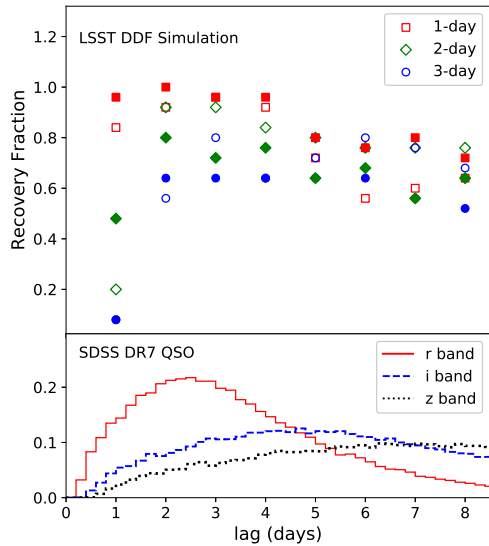
Figure 24. (upper panel) Recovery fraction of time lags from simulated lightcurves in the LSST DDFs as a function of input time lags. The red squares, green diamonds and blue circles represent the result for lightcurves with a 1-day, 2-day and 3-day cadence, respectively. The open symbols represent results from lightcurves with gaps, while filled markers are from lightcurves without gaps. (lower panel) Predicted lag distributions for the SDSS DR7 quasars. The red, blue and black lines represents the lag distribution in the r , i and z band relative to g band, respectively.
