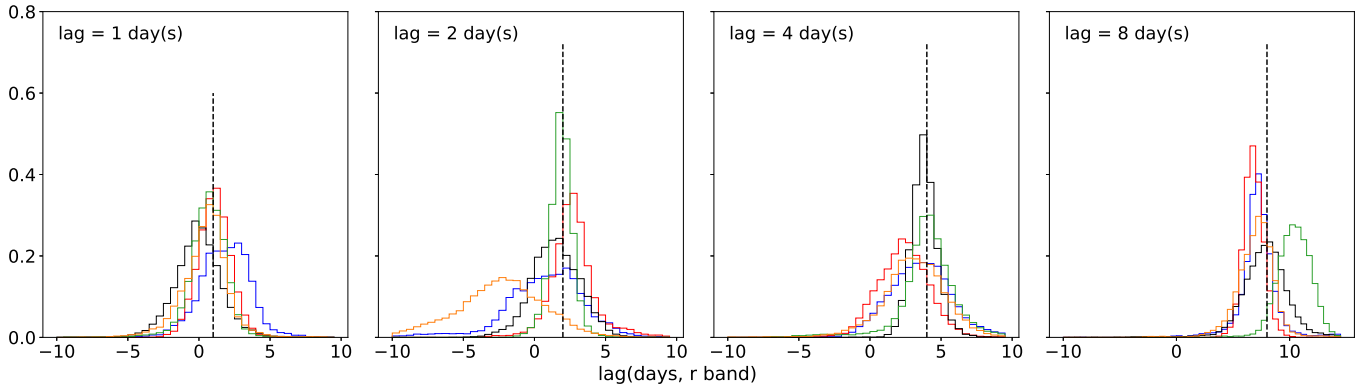
Figure 14. Probability distribution of r -band time lags relative to g -band from fitting the five realizations (LC0 - LC4) of the simulated DRW light curves with the same \sim 1 day cadence as DES J063037.48–575610.30 (same quasar as Figure 13) with ICCF. The histograms with different colors in each panel represent the ICCF center distributions for different realizations of the DRW lightcurves. The black dashed line in each panel represents the position of the input time lag, which is 1, 2, 4 and 8 day(s) for the first, second, third and fourth column, respectively.
