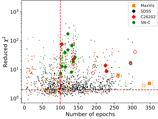
Figure 3. \chi_r^2 as a function of the number of epochs. The orange squares, black circles, red diamonds and green pentagons represent the objects from the MaxVis field, the SDSS fields, the C26202 standard star field, and the SN-C fields, respectively. The small symbols represent the objects where we do not obtain good lag measurements. The large symbols represent the objects in the main sample with the empty symbols for the flagged objects. For the objects without lag measurements, \chi_r^2 and the number of epochs are calculated from the season where \chi_r^2 is the largest. For objects in the main sample, \chi_r^2 and the number of epochs are from the season where the lags and disk sizes are measured. If an object has lag measurements from multiple seasons, \chi_r^2 is from the earliest season that has lag measurements. The horizontal red dashed line is drawn at \chi_r^2 = 2 , and the vertical line is drawn at N_{fit} = 100 .
