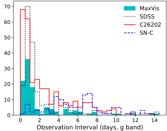
Figure 1. Time interval distribution between consecutive pairs of epochs for the lightcurve of a representative object in each field. The cyan filled, black dotted, red solid and blue dashed histograms are the cadence distribution of DES J063037.48–575610.30 in the MaxVis field, DES J005905.51+000651.66 in the SDSS fields, DES J033408.25–274337.81 in the C26202 field and DES J034001.53–274036.91 in the SN-C fields, respectively.
