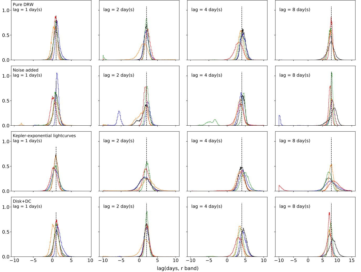
Figure 13. Probability distribution of r -band time lags relative to g -band from fitting the five realizations (LC0 - LC4) of the simulated light curves of DES J063037.48–575610.30 in the MaxVis field. The histograms with different colors in each panel represent the JAVELIN result for different realizations of the simulated lightcurves. The black dashed line in each panel represents the position of the input time lag, which is 1, 2, 4 and 8 day(s) for the first, second, third and fourth column, respectively. The first through the fourth row represent the results from pure DRW lightcurves, DRW lightcurves with noise, Kepler-exponential lightcurves and the composite lightcurves of the accretion disk and the diffuse continuum from the BLR.
