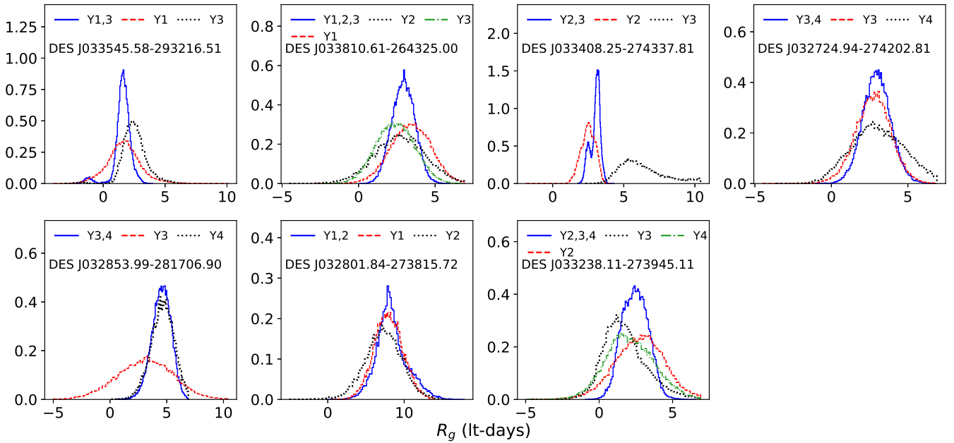
Figure 11. Probability distributions for the observed frame g -band accretion disk sizes from the JAVELIN Thin Disk model for objects with multi-season lag measurements. In each panel the blue solid line represents the results of a simultaneous fit to all observational seasons with lag measurements, while the red dashed, black dotted and green dash-dotted lines represent the results for individual seasons.
