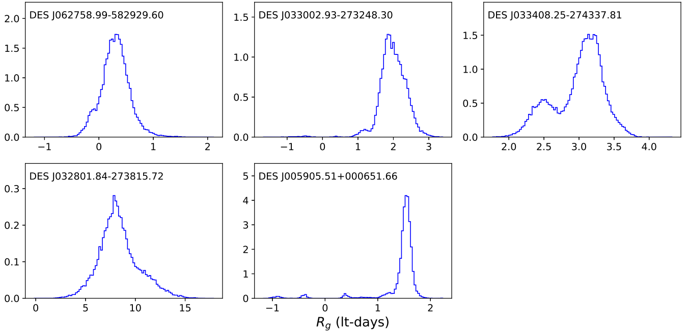
Figure 10. Same as Figure 9, but for quasars with flags in the main sample.
