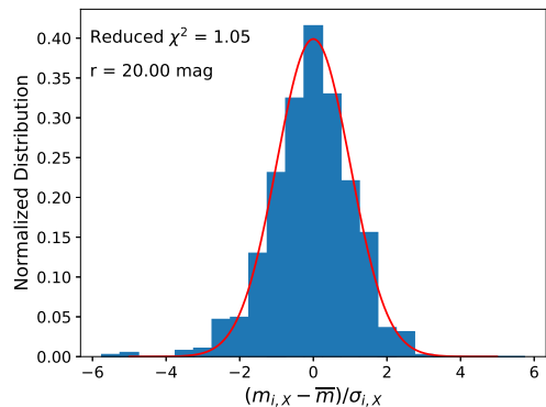
Figure 17. Example of the “Gaussianity” of the DES photometric errors. The blue histograms show the distribution of (m_{i,X} - \bar{m}_X) / \sigma_{i,X} for a standard star. The red line shows a Gaussian profile centered at 0 with a standard deviation equal to 1. The upper left corner shows \chi_r^2 value (see Section 4.3) and the r -band magnitude of the star.
