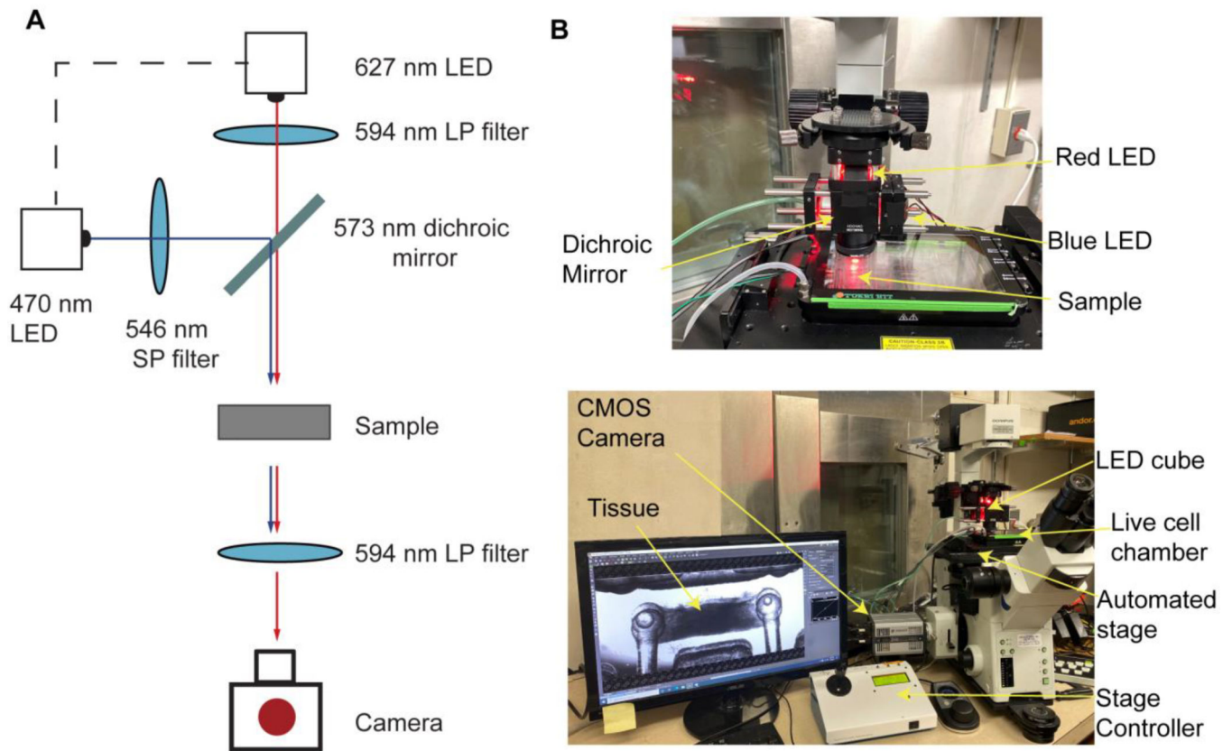
Figure 4. Optical set-up for simultaneous stimulation and recording of engineered NMJs. (A) Light path (B) Implementation of the custom optical set-up in a traditional inverted microscope provided with a live cell chamber, an automated stage and a CMOS camera.
