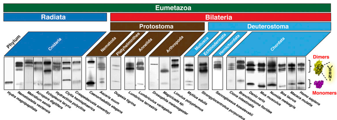
Fig. 3. NC1 hexamers were excised from animal basement membranes and analyzed by SDS/PAGE as shown in Fig. 1 A and B. The dimeric subunits, which indicate the presence of the bond, were found in nine major eumetazoan phyla. Among eight cnidarians investigated, only Hydra NC1 lacked dimeric subunits. All NC1s were immunoblotted against the rat monoclonal antibody, JK2, except for C. elegans (rabbit polyclonal; NW-154) and Drosophila (mouse monoclonal; 6G7). Black outlines indicate the locations of cropping for blot images.
