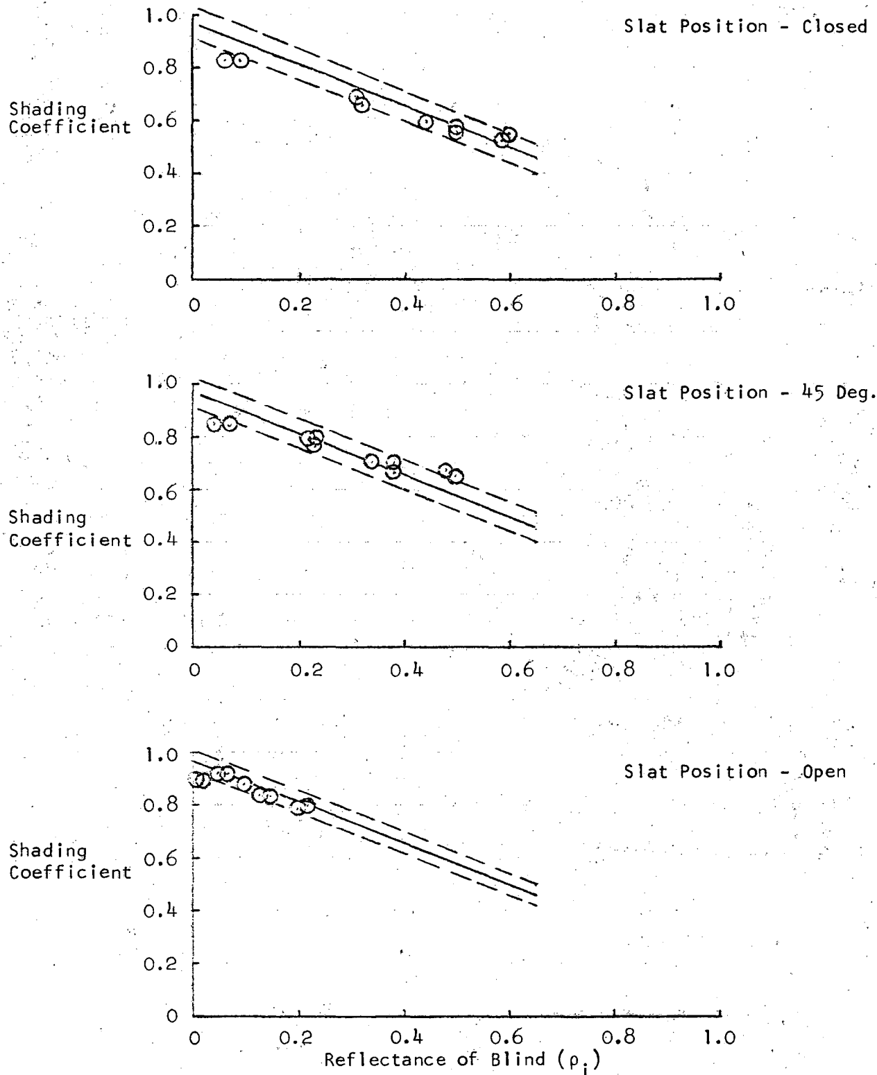
FIGURE 6. COMPARISON OF PREDICTED AND MEASURED SHADING COEFFICIENTS One-Inch Blinds with 1/4-Inch Clear Glass 35 Deg. Solar Incidence Angle Still Air Conditions
