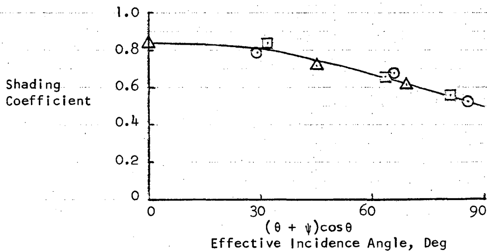
FIGURE 12. SHADING COEFFICIENT AS A FUNCTION OF EFFECTIVE INCIDENCE ANGLE
