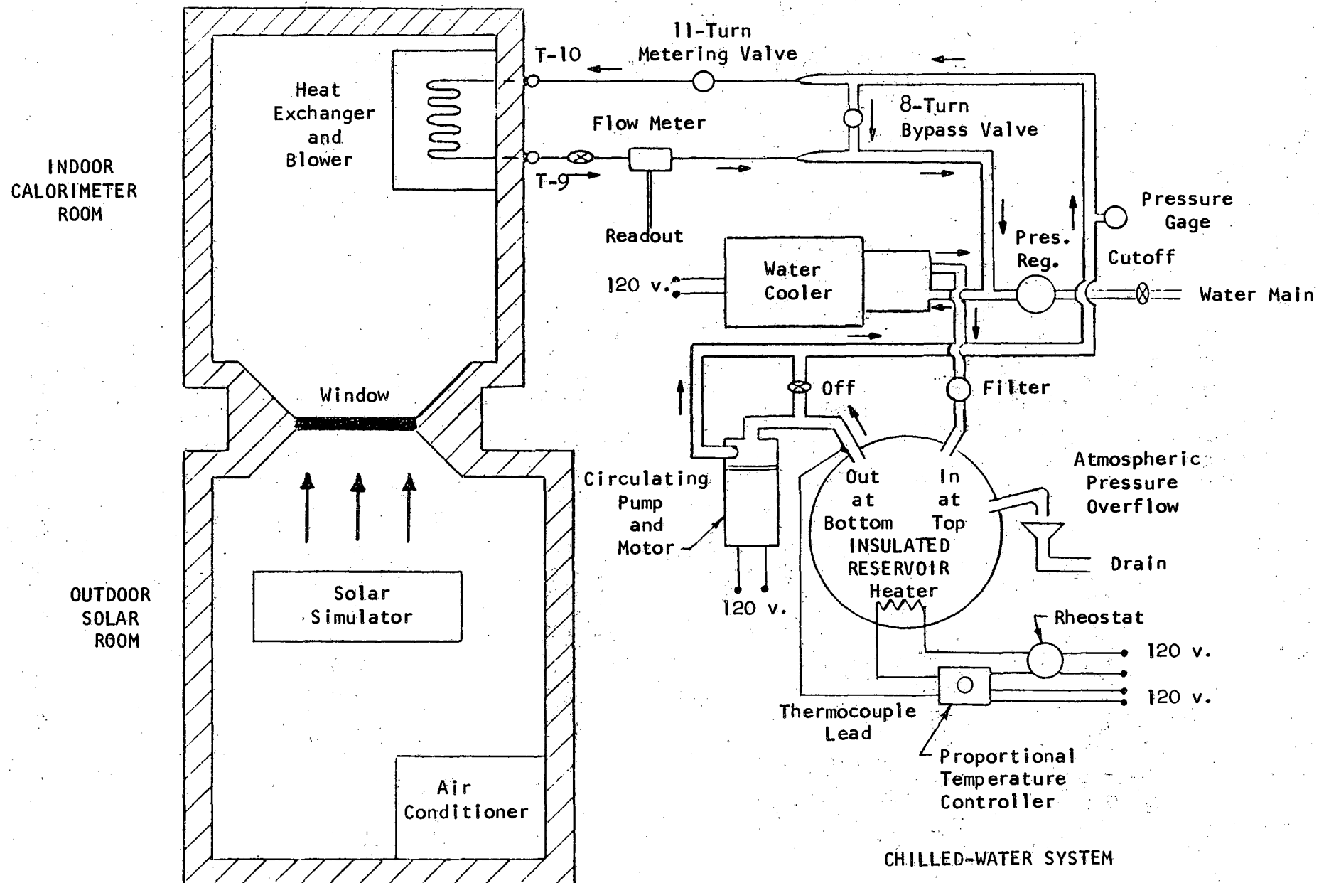
FIGURE 2. LEVOLOR ENVIRONMENTAL SIMULATOR
