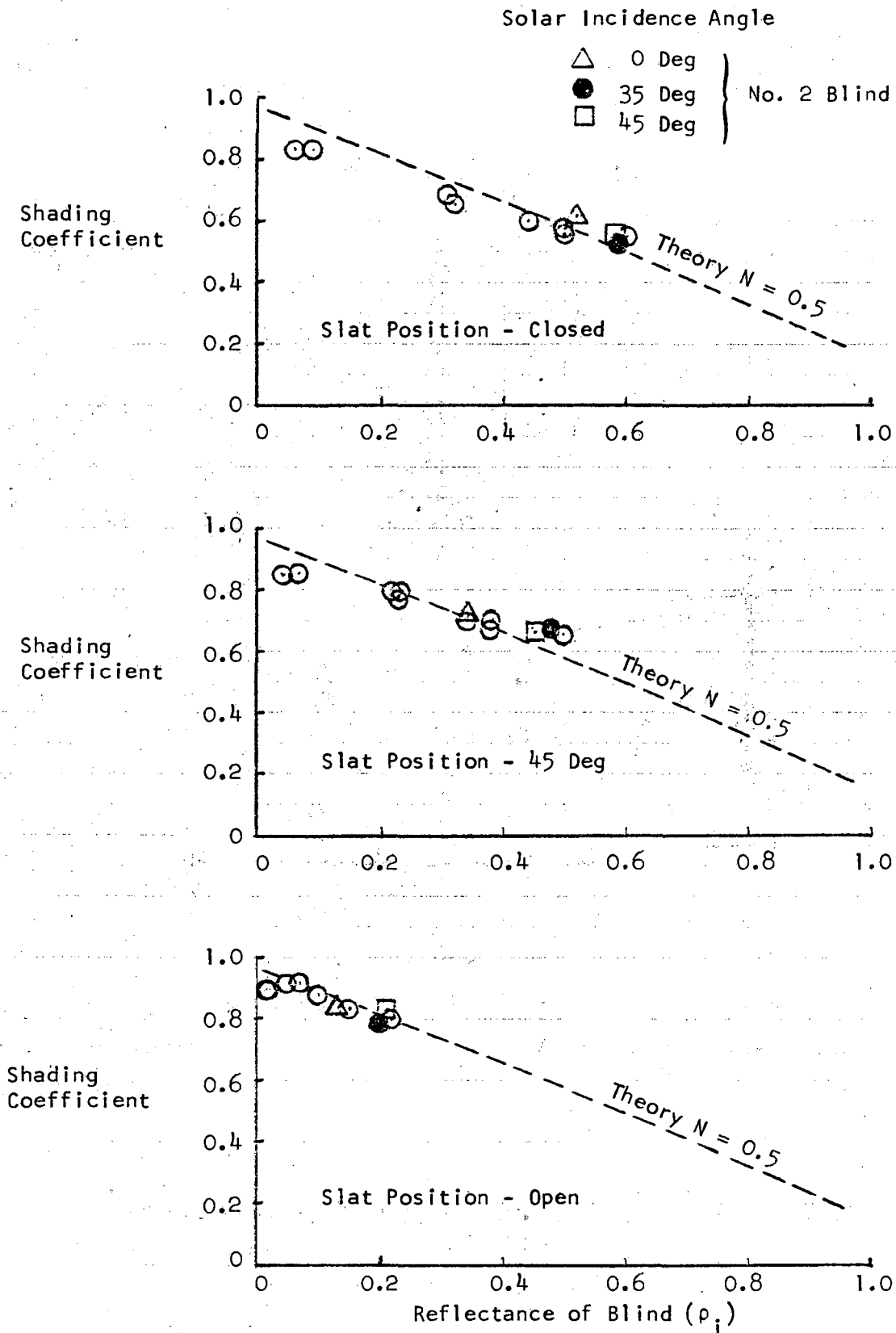
FIGURE 10. EFFECT OF BLIND REFLECTANCE ON SHADING COEFFICIENT Measured in Environmental Simulator - Still Air One Inch Blinds With 1/4-Inch Clear Glass
