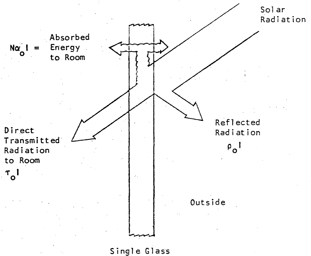
FIGURE 1. HEAT TRANSFER THROUGH SELECTED GLAZING SYSTEMS
