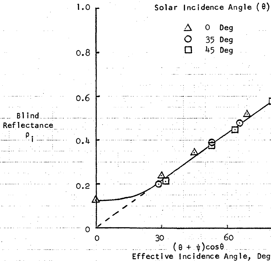
FIGURE 11. EFFECT OF SLAT ANGLE AND SOLAR INCIDENCE ON BLIND REFLECTANCE
