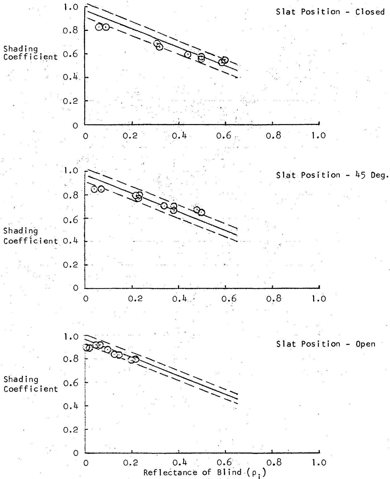
FIGURE 6. COMPARISON OF PREDICTED AND MEASURED SHADING COEFFICIENTS
