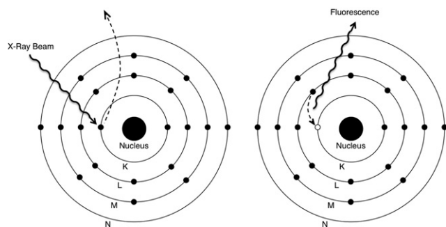
Figure 1. XRF in calcium. Incoming x-ray photon excites core shell electron of atom, in this case K-shell electron. Core hole is filled by 1 outer electron and extra energy, which is binding energy difference of 2 shells, is released as fluorescence radiation. Since electron binding energies are element specific, analyzing fluorescence energy can be used to determine atomic composition of its source. Calcium photoionization and subsequent fluorescence emission shown resulted in calcium K peak of 3,690 eV energy (K and L electron binding energies were 4,038.5 and 348.5 eV, respectively). To generate calcium K peak energy of incoming x-ray beam must be higher than 4,038.5 eV (fig. 3). X-ray emission peaks are labeled based on shell from which they originated. L, M and N, electron shells.
