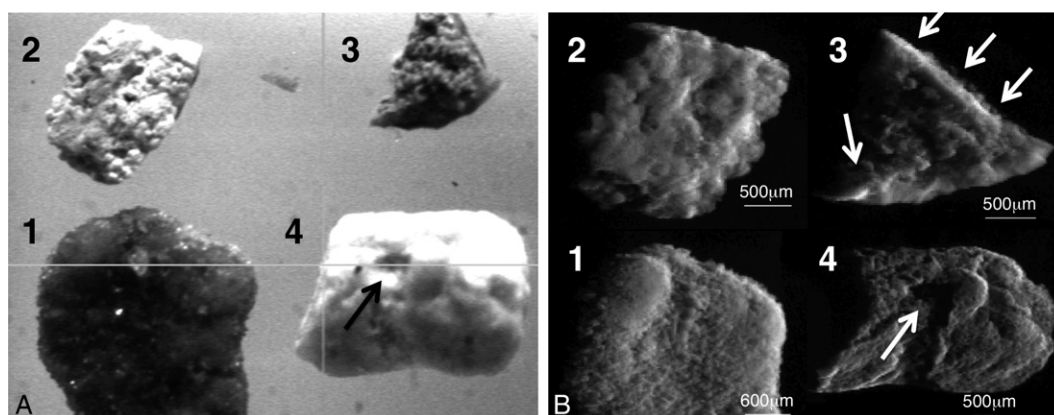
Figure 4. A, detailed image of stone samples mounted on beamline x-y stage. B, \mu XRF elemental maps reveals calcium distribution with image brightness proportional to calcium signal strength. Data were collected at 1,6205 eV x-ray energy, 20 \mu m pixel size and 15 \times 6 \mu m beam spot size. Left edge shows weaker calcium fluorescence signal for all 4 maps due to shadowing effect caused by experimental geometry. Similarly, signal from indentation (arrow) in sample 4 was weakened by protrusion at right. Sample 3 was composite stone (see table), resulting in uneven calcium distribution. Note strong calcium signal on upper and lower edges (arrows). Scale bars indicate 600 (sample 1) and 500 (samples 2 to 4) \mu m.
