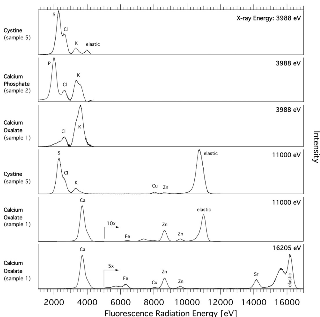
Figure 3. XRF spectra of representative stone samples collected at 3 x-ray energies. Calcium containing stones showed strong calcium K peak at 3,690 eV as long as exciting x-ray energy was above K-shell ionization threshold, also known as K-edge, of 4,038.5 eV. Second and third spectra showed no calcium signal because x-ray excitation energy was below calcium core shell ionization energy, thus, deliberately excluding calcium measurement. Purpose was to see signal from other elements, such as phosphorus for apatite stone, which would be masked by strong calcium peak. Cystine sample shows strong sulfur K peak. Due to \mu XRF method high sensitivity, trace elements chlorine, potassium, iron, zinc, copper and strontium were also observed. Elastic peak represents incoming x-ray beam, which was scattered without energy loss.
