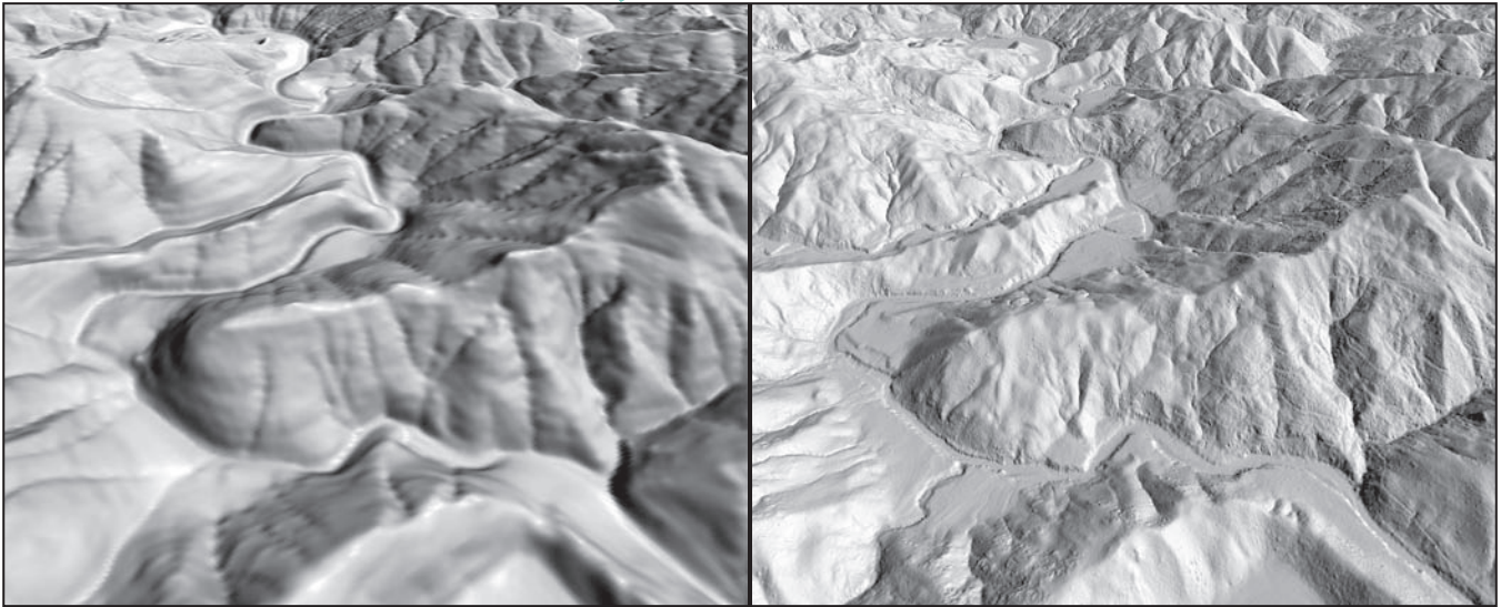
A COMPARISON OF STANDARD TOPOGRAPHIC MAPPING AND LIDAR IMAGES. THE DETAIL SHOWN ON THE LEFT IS A 10M DEM (DIGITAL ELEVATION MODEL) TAKEN FROM A USGS 7.5' QUAD. IT SEEMS BLURRED AND INACCURATE WHEN COMPARED WITH A CRISP 1M DEM OF THE SAME AREA CREATED THROUGH AIRBORNE LASER-SWATH MAPPING. IMAGES COURTESY OF THE NATIONAL CENTER FOR EARTH-SURFACE DYNAMICS (NCED)
