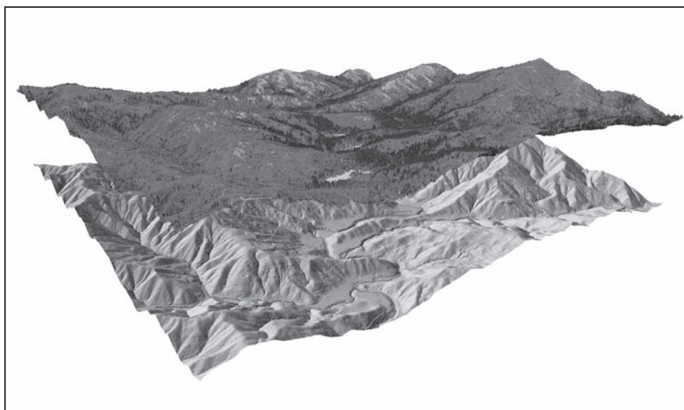
THIS THREE-DIMENSIONAL LIDAR MAP REVEALS, IN GREAT DETAIL, A PORTION OF THE NRS'S ANGELO RESERVE — BOTH "CLOTHED" AND "UNCLOTHED." IMAGE COURTESY OF THE NATIONAL CENTER FOR EARTH-SURFACE DYNAMICS (NCED)
