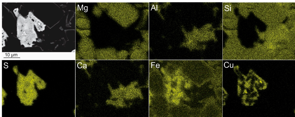
Figure 5. SEM-EDS maps displaying the elemental abundance in a small area highlighted in Figure 4b. First image is SEM-BSE. Areas rich in Al, Ca and Si correspond to the amorphous matrix. High brightness in Cu is elemental copper.
