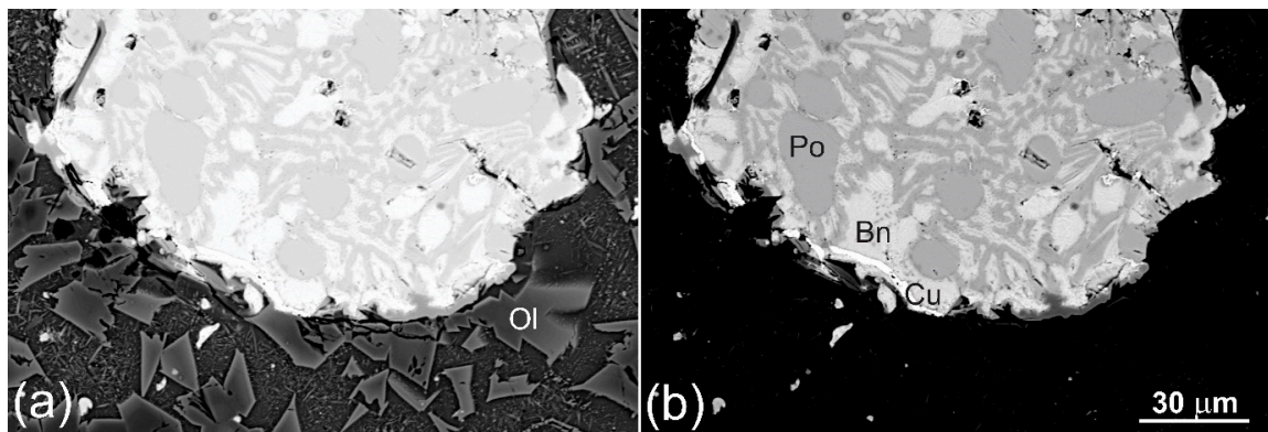
Figure 6. SEM-BSE images of a sample of non-magnetic slag (Figure 2e). Cu-Fe sulfide nodule (bright) composed of pyrrhotite (Po), bornite (Bn) and elemental copper (Cu, white line) in a matrix of zoned prismatic olivine (Ol) crystals. Both images are of the same area and the same magnification (scale in (b) applies to both figures) but (a) is at high brightness to emphasize olivine microstructure and (b) at lower brightness to display complex intergrowth structures of sulfides.
