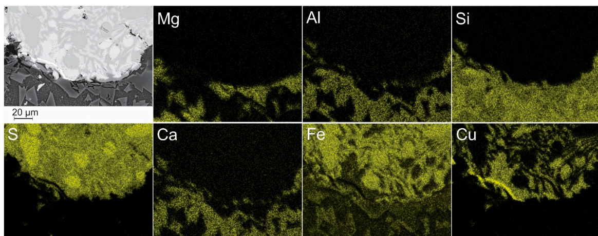
Figure 7. SEM-EDS maps displaying the elemental abundance in the area displayed in Figure 6. First image is SEM-BSE. Areas rich in Al, Ca and Si correspond to the amorphous matrix. High brightness in Cu map is elemental copper and medium brightness is bornite.
