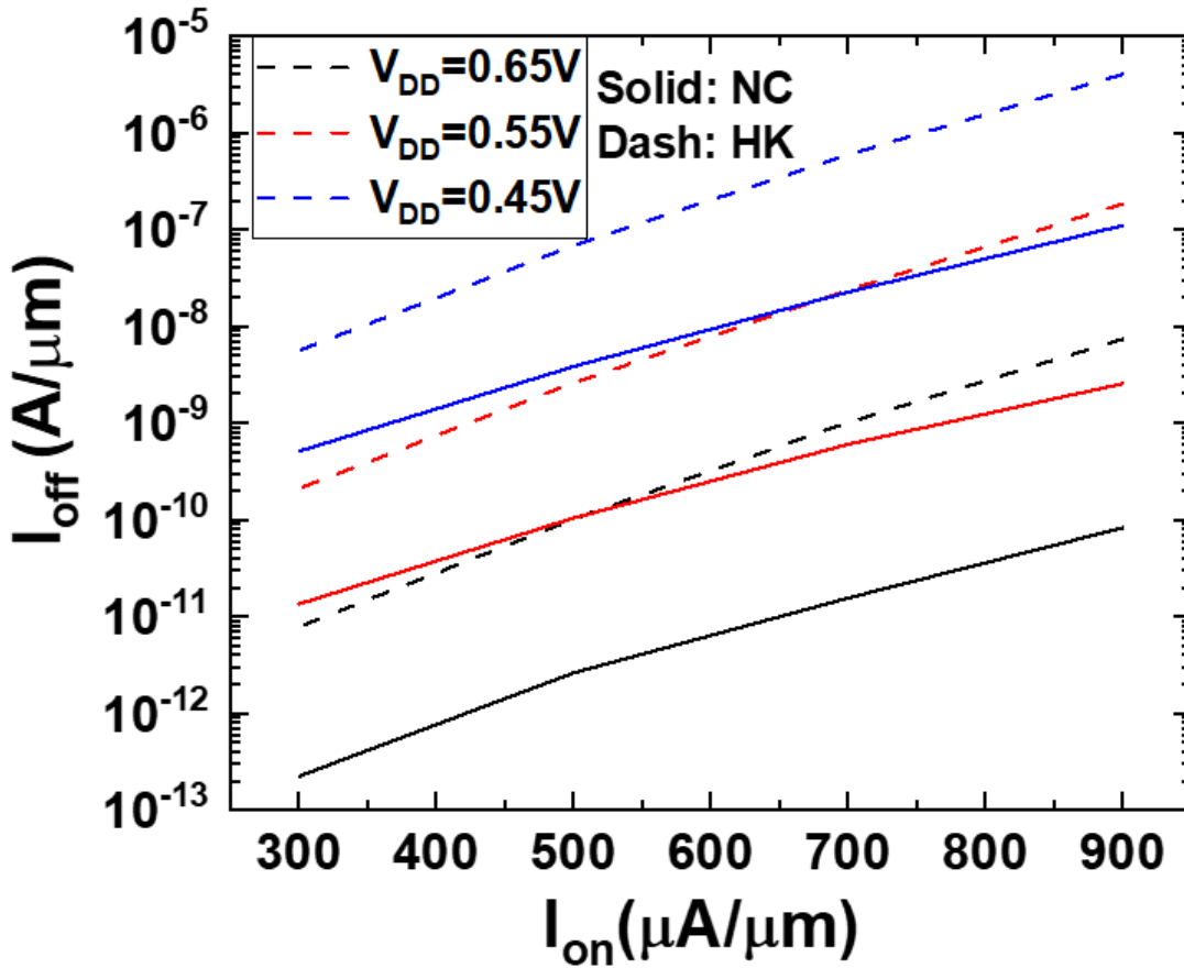
Fig. 7.5. I_{off} - I_{on} plot of HK-GAA (dash lines) and NC-GAA (solid lines) under different V_{DD} conditions. NC-GAA with V_{DD} of 0.55V (solid red line) performs even better than HK-GAA with V_{DD} of 0.65V (dashed black line) in the high-performance region ( I_{on} > 550 \mu A/\mu m ).
