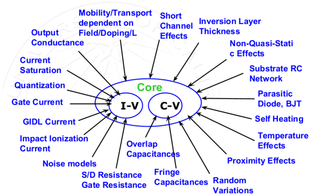
Fig. 1.4. Architecture of BSIM from Prof. Chenming Hu's presentation in Sep. 2013.
