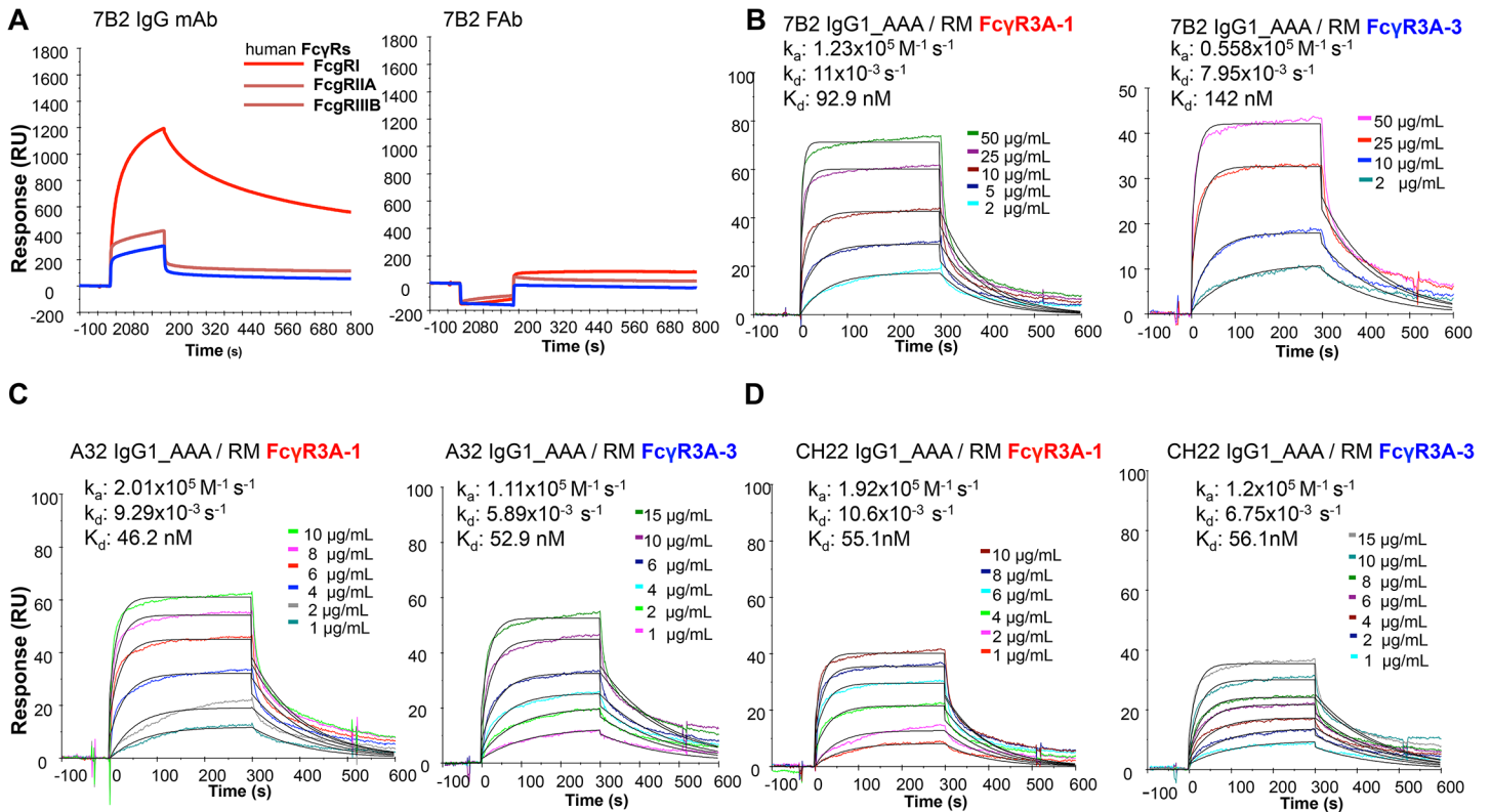
Fig 2. Surface plasmon resonance of mAbs to human and rhesus FcR. (A) 7B2 IgG1_ AAA and Fab to human FcR FcγRI, FcγRIIA, FcγRIIIB and (B) rhesus macaque FcγR3A-1 and _FcγR3A-3. (C) A32 IgG1_ AAA and (D) CH22 IgG1_ AAA to rhesus macaque FcγR3A-1 and _FcγR3A-3.
