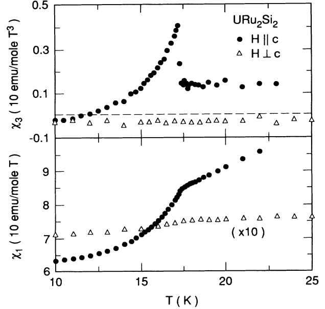
FIG. 2. Nonlinear susceptibility \chi_3 and linear susceptibility \chi_1 for URu 2 Si 2 . The response is shown for both the easy magnetic direction, parallel to the tetragonal c axis (solid symbols), and in the hard direction perpendicular to the c axis (open symbols). The peak in \chi_3 at the same temperature where the specific heat peaks illustrates the predominance of high-order spin correlations for establishing magnetic order.
