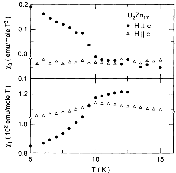
FIG. 3. Nonlinear susceptibility \chi_3 and linear susceptibility \chi_1 for U 2 Zn 17 . The response is shown for both the easy magnetic direction perpendicular to the rhombohedral c axis (solid symbols) and in the hard direction parallel to the c axis (open symbols). The vanishing of \chi_3 near T_N is the expected behavior for a conventional antiferromagnet.
