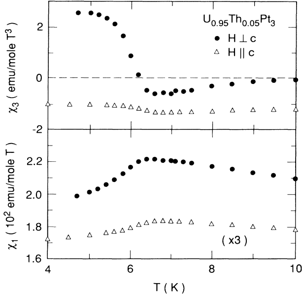
FIG. 4. Nonlinear susceptibility \chi_3 and linear susceptibility \chi_1 for \text{U}_{0.95}\text{Th}_{0.05}\text{Pt}_3 . The response is shown for both the easy magnetic direction, perpendicular to the hexagonal c axis (solid symbols) and in the hard direction, parallel to the c axis (open symbols). The vanishing of \chi_3 near T_N is the expected behavior for a conventional antiferromagnet.
