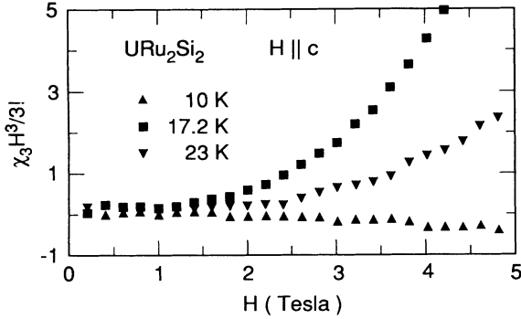
FIG. 1. The leading nonlinear term, \chi_3 H^3/3! , in the magnetization of URu 2 Si 2 , for H parallel to the tetragonal c axis, at three different temperatures spanning the transition at 17.3 K.
