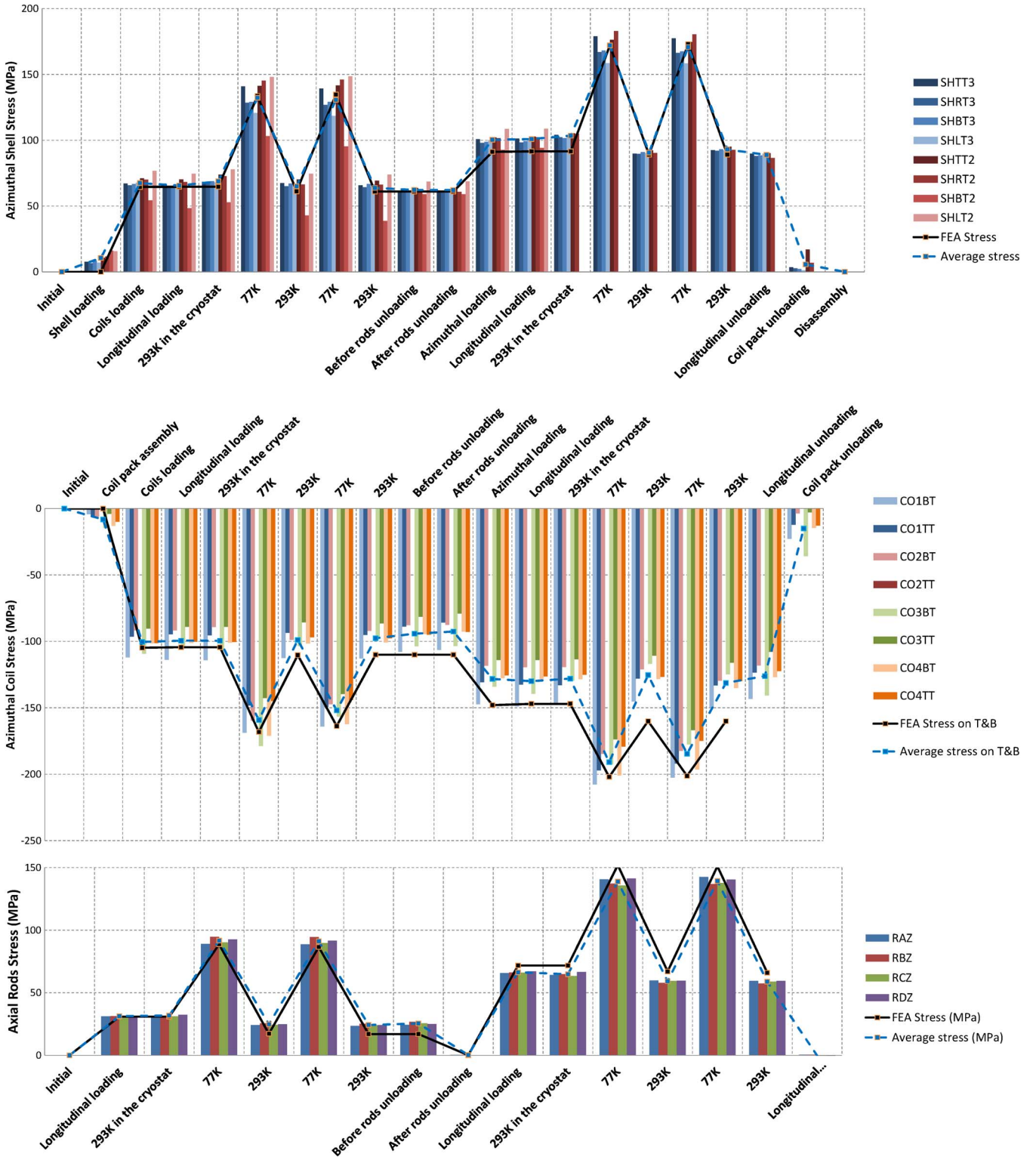
Fig. 6. (top) Azimuthal stress in aluminum shells, (middle) azimuthal stress in the dummy coils, and (bottom) axial stress in the rods of the CERN structure MQXFSD0 at the consecutive test steps. The state of the dummy coil is presented in the location corresponding to the center of the shell segment ("Top" and "Bottom" coil strain gauges in Fig. 3).
