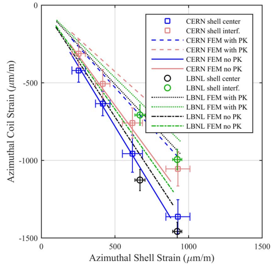
Fig. 5. Room-temperature loading behavior of the CERN and the LBNL structure. Measurement data are shown in the area corresponding to the center of the shell segment (“Top” and “Bottom” coil strain gauges in Fig. 3) and in the area corresponding to the interface between two shells segments (“Mid” coil strain gauges). The results of the FEM analysis are shown for the same locations. Two different FEM models were analyzed for each structure, with and without pole keys (PK) between the collars.
