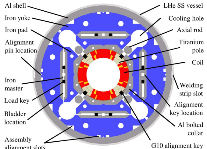
Fig. 1. MQXF magnet cross section.
