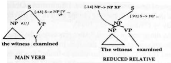
Figure 3: The syntactic parse trees for the MV and the RR interpretations assuming an SCFG generating grammar.
