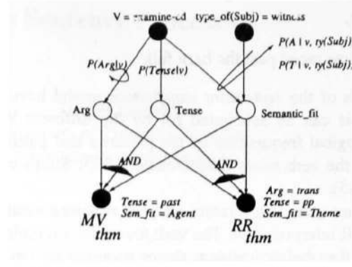
Figure 2: The Belief net that represents lexical support for the two interpretations for the same input. The input is from data in Table 1.
