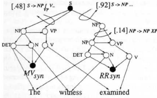
Figure 4: The Belief network corresponding to the syntactic support.
