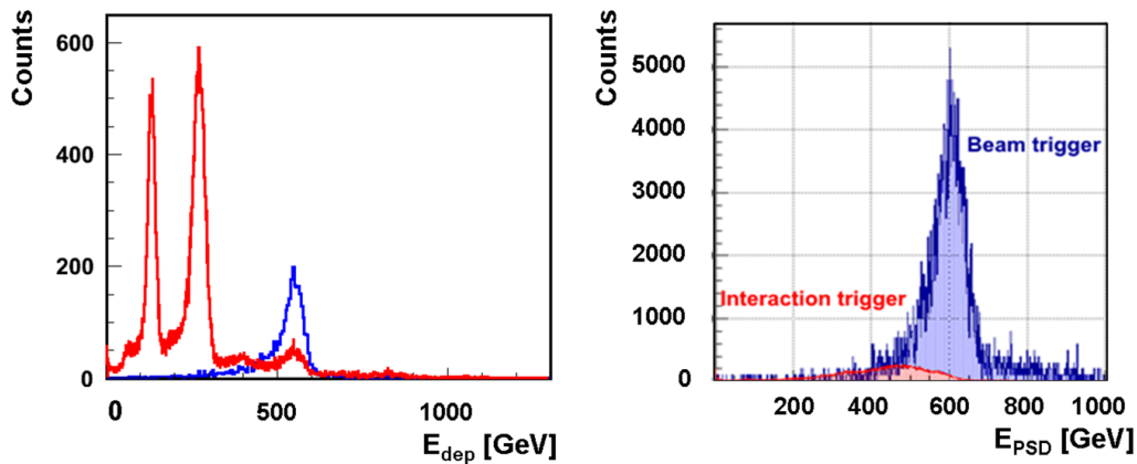
Figure 28. Left: PSD energy distributions for the secondary ion beam at 75A GeV/ c with and without selection of the {}^7\text{Be} ions by the Z-detector. Right: PSD energy distributions recorded during the data taking for {}^7\text{Be}+{}^9\text{Be} interactions at 75A GeV/ c . Spectra are shown for the beam trigger (blue) and for the interaction trigger (red) events.
