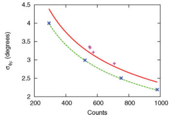
Fig. 7. A comparison of the phase uncertainty for fluorescein measurements as a function of counts between a Becker & Hickl card Model 830 on an 80 MHz 2-photon system (solid line, + symbol) and the FLIMBox on a diode laser system driven at 48 MHz (dashed line, x symbol). Per equal counts, the uncertainty for the B&H card is higher than the FLIMBox card due to the increased demodulation of the fluorescein signal at 80 MHz with respect to 48 MHz. However, all the uncertainties are close to the values predicted by the mathematical model when this demodulation is taken into account. [Color figure can be viewed in the online issue, which is available at www.interscience.wiley.com .]
